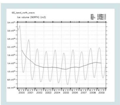
ICE_icevol_north
