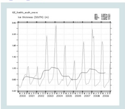
ICE_icethic_south
