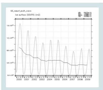
ICE_icesurf_south
