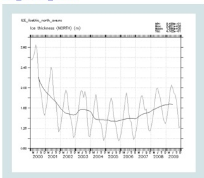
ICE_icethic_north
