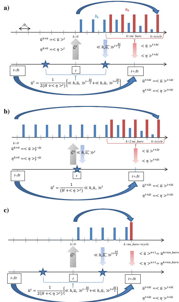
FIG. 6.2: Schematic of the split-explicit time stepping scheme for the external and internal modes. Time increases to the right. In this particular example, a box-car averaging window over nn\_baro barotropic time steps is used ( nn\_bt\_filt = 1 ) and nn\_baro = 5 . Internal mode time steps (which are also the model time steps) are denoted by t - \Delta t , t and t + \Delta t . Variables with k superscript refer to instantaneous barotropic variables, \langle \rangle and \langle \langle \rangle \rangle operator refer to time filtered variables using respectively primary (red vertical bars) and secondary weights (blue vertical bars). The former are used to obtain time filtered quantities at t + \Delta t while the latter are used to obtain time averaged transports to advect tracers. a) Forward time integration : ln\_bt\_fw=true , ln\_bt\_ave=true . b) Centred time integration : ln\_bt\_fw=false , ln\_bt\_ave=true . c) Forward time integration with no time filtering (POM-like scheme) : ln\_bt\_fw=true , ln\_bt\_ave=false .
