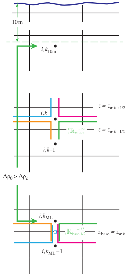
FIG. E.4: Definition of mixed-layer depth and calculation of linearly tapered triads. The figure shows a water column at a given i, j (simplified to i ), with the ocean surface at the top. Tracer points are denoted by bullets, and black lines the edges of the tracer cells; k increases upwards.
