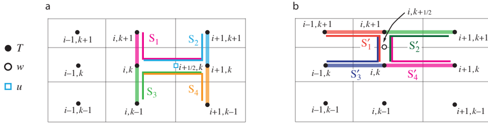
FIG. E.1: (a) Arrangement of triads S_i and tracer gradients to give lateral tracer flux from box i, k to i + 1, k (b) Triads S'_i and tracer gradients to give vertical tracer flux from box i, k to i, k + 1 .
