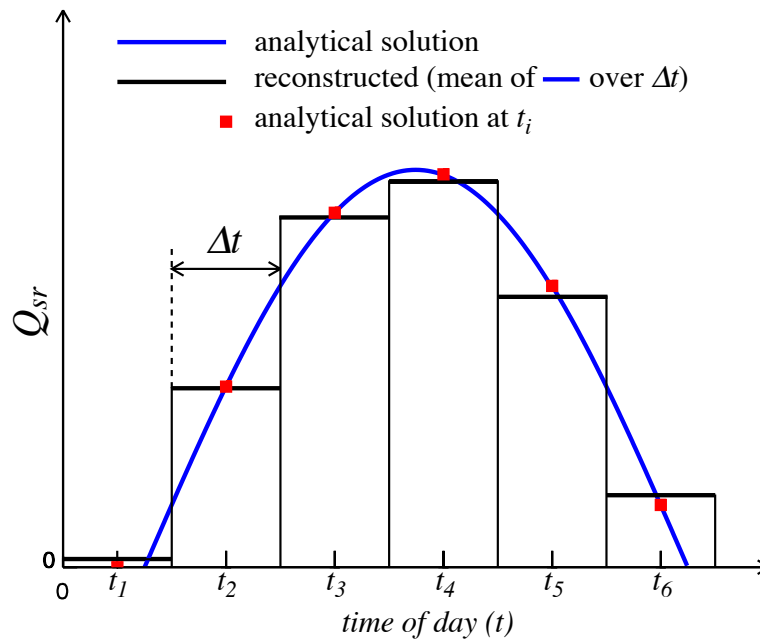
FIG. 7.1: Example of reconstruction of the diurnal cycle variation of short wave flux from daily mean values. The reconstructed diurnal cycle (black line) is chosen as the mean value of the analytical cycle (blue line) over a time step, not as the mid time step value of the analytically cycle (red square). From ?.
