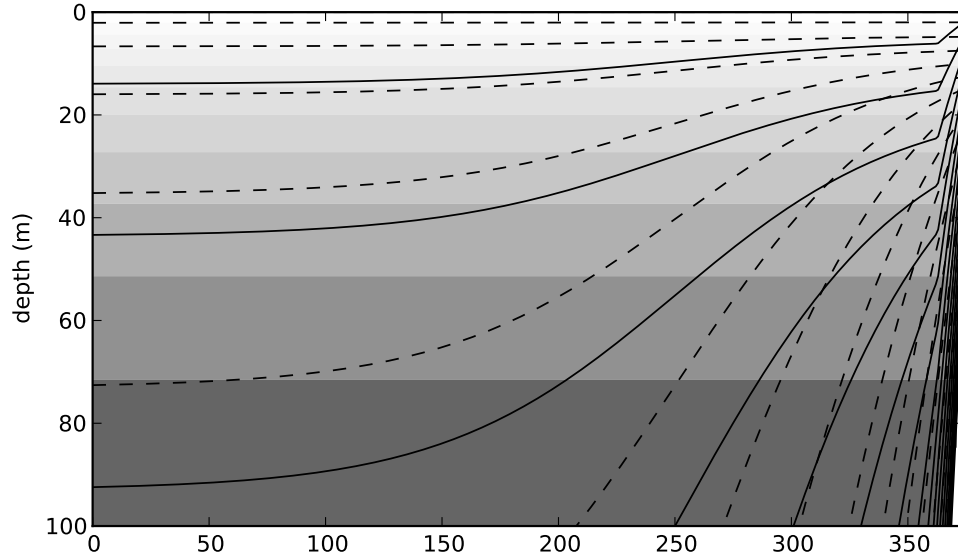
FIG. 4.8: A comparison of the \sigma S -coordinate (solid lines), a 50 level Z -coordinate (contoured surfaces) and the \sigma S -coordinate (dashed lines) in the surface 100m for a idealised bathymetry that goes from 50m to 5500m depth. For clarity every third coordinate surface is shown.
