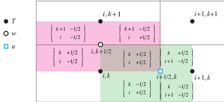
FIG. E.2: Triad notation for quarter cells. T -cells are inside boxes, while the i + \frac{1}{2}, k u -cell is shaded in green and the i, k + \frac{1}{2} w -cell is shaded in pink.
