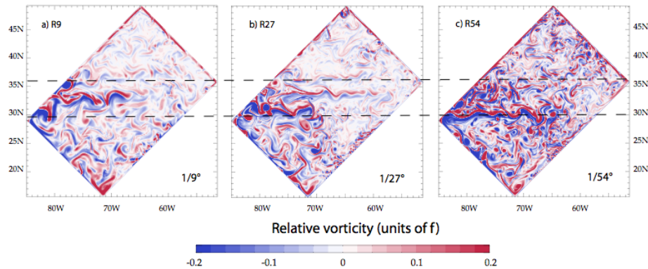
Figure 16.3: Snapshot of relative vorticity at the surface of the model domain in GYRE R9, R27 and R54. From Lévy et al. [2010].
