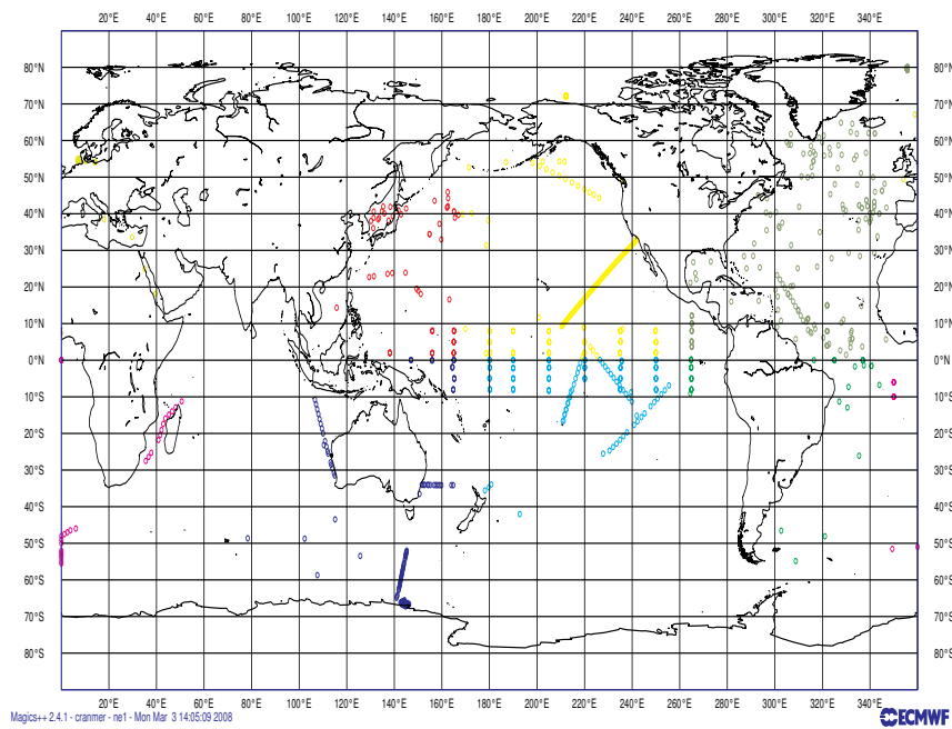
Figure 12.3: Example of the distribution of observations with the geographical distribution of observational data.
