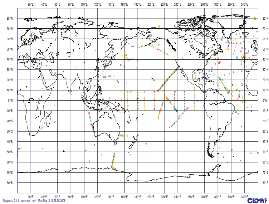
Figure 12.4: Example of the distribution of observations with the round-robin distribution of observational data.
