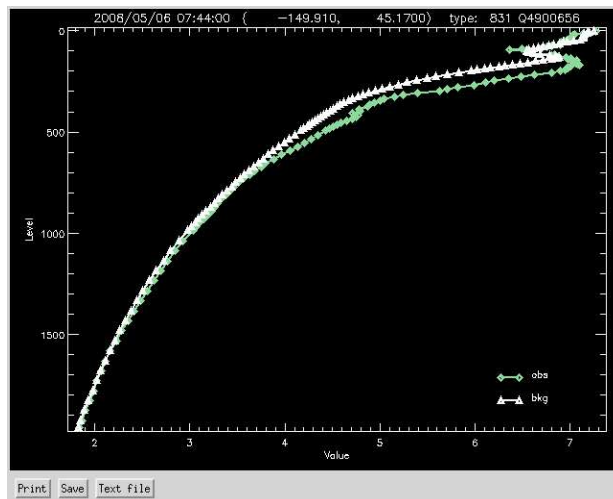
Figure 12.6: Profile plot from dataplot produced by right clicking on a point in the main window.
