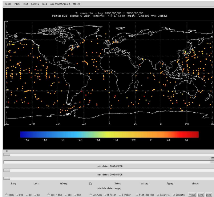
Figure 12.5: Main window of dataplot.
