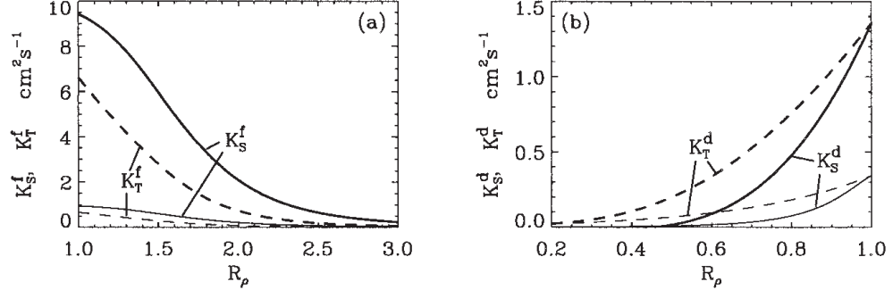
FIG. 9.3 – From Merryfield et al. [1999] : (a) Diapycnal diffusivities A_f^{vT} and A_f^{vS} for temperature and salt in regions of salt fingering. Heavy curves denote A^{*v} = 10^{-3} m^2.s^{-1} and thin curves A^{*v} = 10^{-4} m^2.s^{-1} ; (b) diapycnal diffusivities A_d^{vT} and A_d^{vS} for temperature and salt in regions of diffusive convection. Heavy curves denote the Federov parameterization and thin curves the Kelley parameterization. The latter is not implemented in NEMO .
