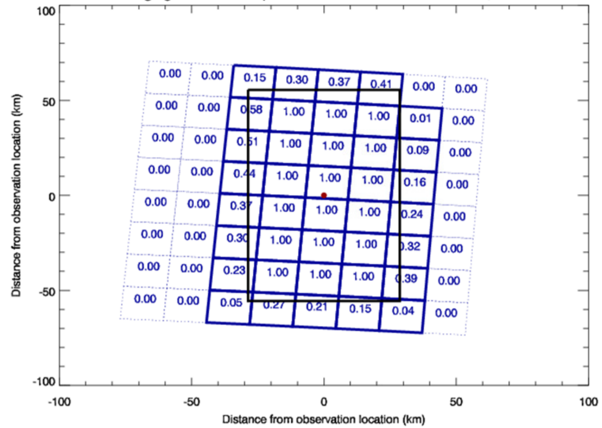
Averaging observation operator for ob centred on: -177.50E, 58.50N
