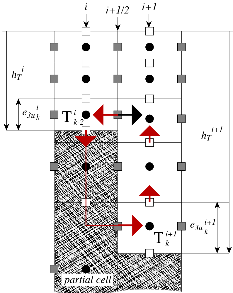
FIG. 4.3 – Advective Bottom Boundary Layer.
