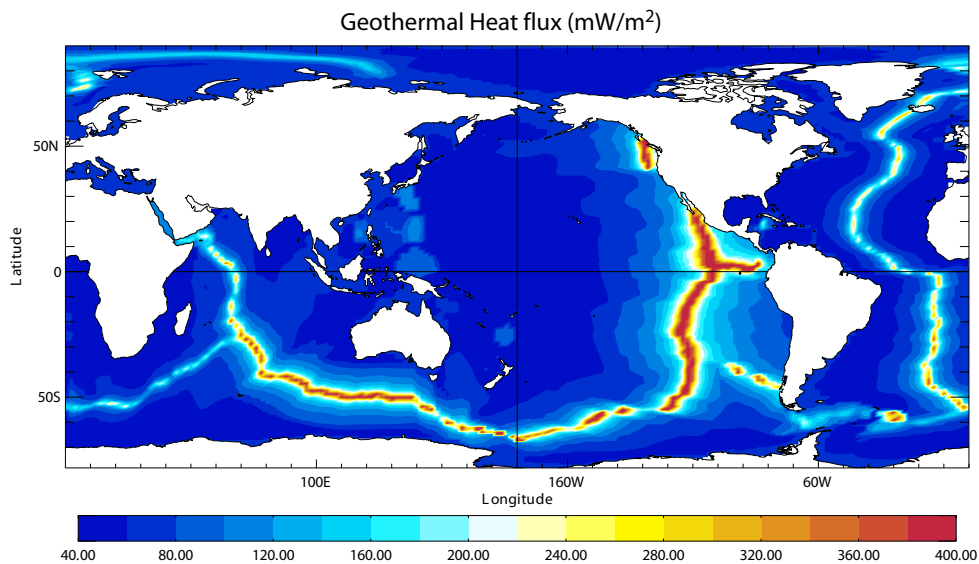
FIG. 4.2 – Geothermal Heat flux (in mW.m^{-2} ) used by Emile-Geay and Madec [2009]. It is inferred from the age of the sea floor and the formulae of Stein and Stein [1992].
