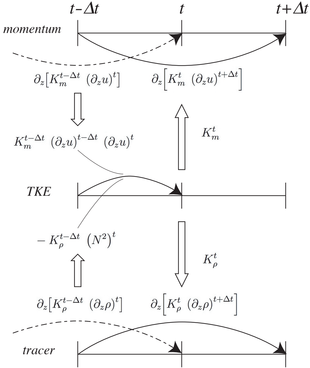
FIG. 9.2 – Illustration of the TKE time integration and its links to the momentum and tracer time integration.
