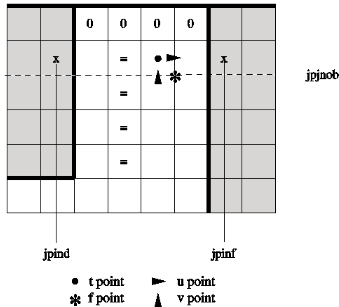
FIG. 7.7 – Localization of the North open boundary points.
