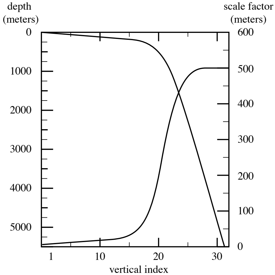
FIG. 3.6 – Default vertical mesh for ORCA2 : 30 ocean levels (L30). Vertical level functions for (a) T-point depth and (b) the associated scale factor as computed from (3.13) using (3.14) in z -coordinate.
