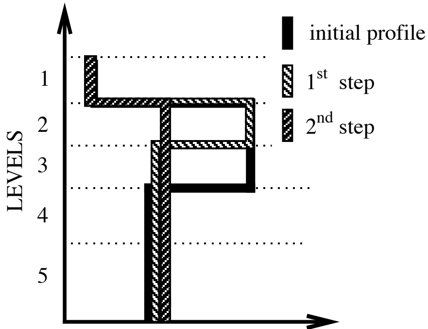
FIG. 9.3 – Example of an unstable density profile treated by the non penetrative convective adjustment algorithm. 1 st step : the initial profile is checked from the surface to the bottom. It is found to be unstable between levels 3 and 4. They are mixed. The resulting \rho is still larger than \rho(5) : levels 3 to 5 are mixed. The resulting \rho is still larger than \rho(6) : levels 3 to 6 are mixed. The 1 st step ends since the density profile is then stable below the level 3. 2 nd step : the new \rho profile is checked following the same procedure as in 1 st step : levels 2 to 5 are mixed. The new density profile is checked. It is found stable : end of algorithm.
