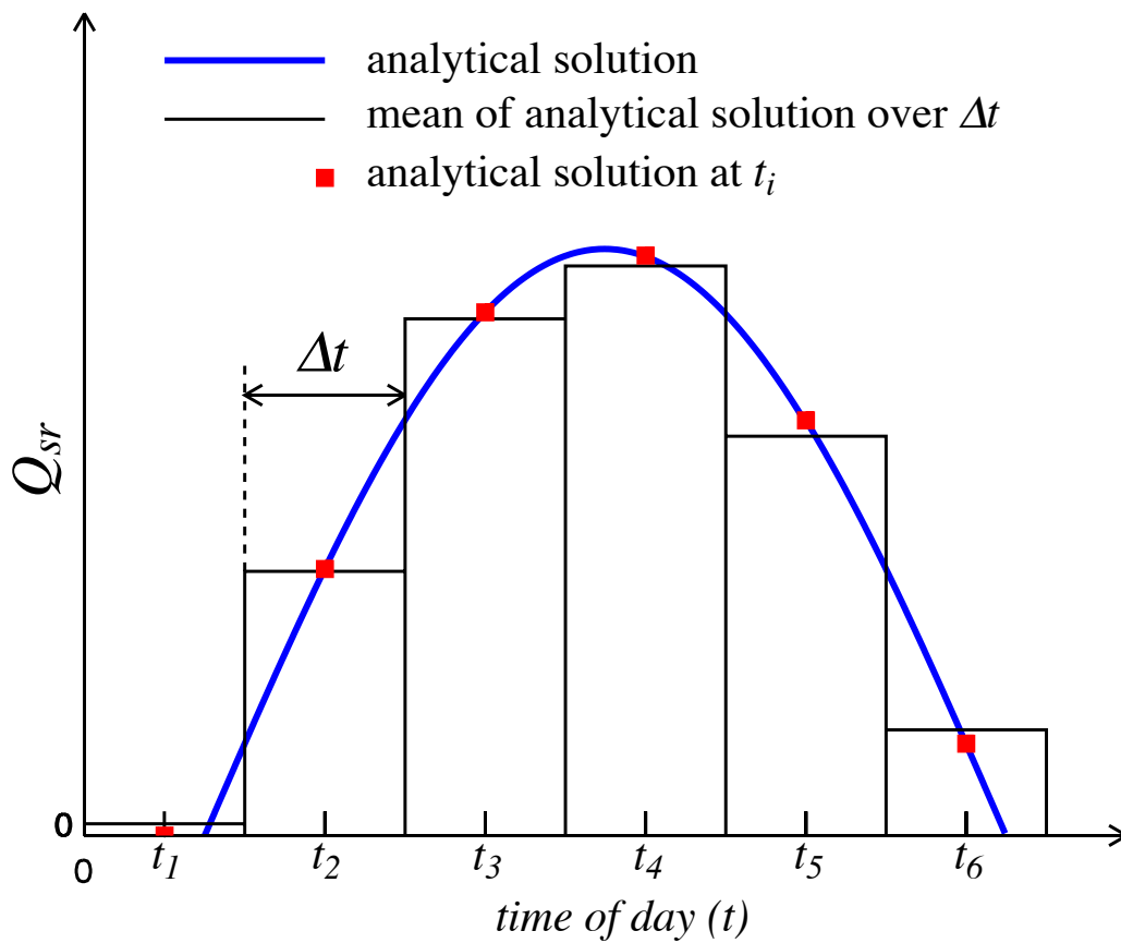
FIG. 7.1 – Example of reconstruction of the diurnal cycle variation of short wave flux from daily mean values. From ?.
