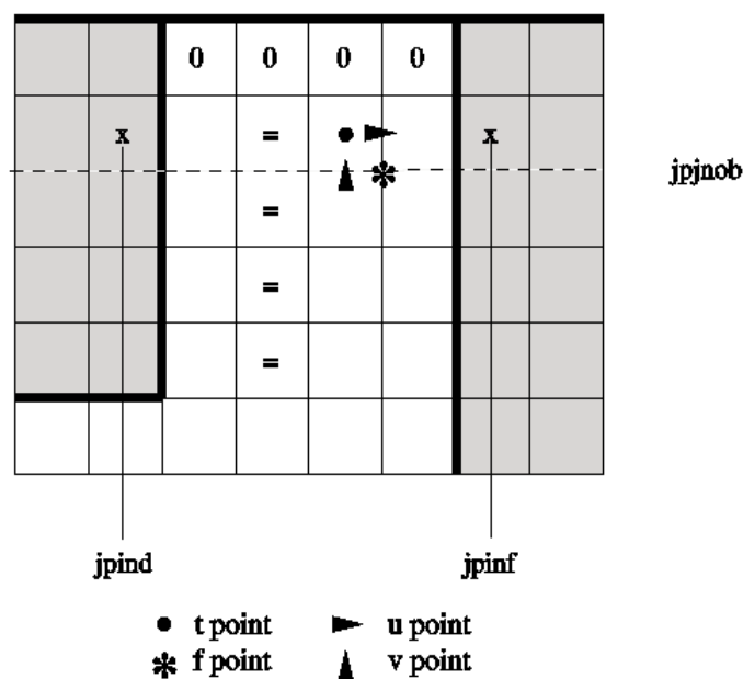
FIGURE 8.7 – Localization of the North open boundary points.
