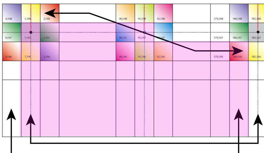
FIGURE 8.4 – North fold boundary with a T -point pivot and cyclic east-west boundary condition ( j_{perio} = 4 ), as used in ORCA 2, 1/4, and 1/12. Pink shaded area corresponds to the inner domain mask (see text).
