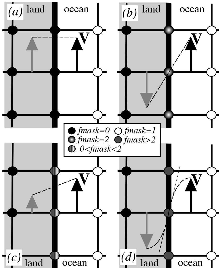
FIGURE 8.2 – lateral boundary condition (a) free-slip ( rn\_shlat = 0 ); (b) no-slip ( rn\_shlat = 2 ); (c) "partial" free-slip ( 0 < rn\_shlat < 2 ) and (d) "strong" no-slip ( 2 < rn\_shlat ). Implied "ghost" velocity inside land area is display in grey.
