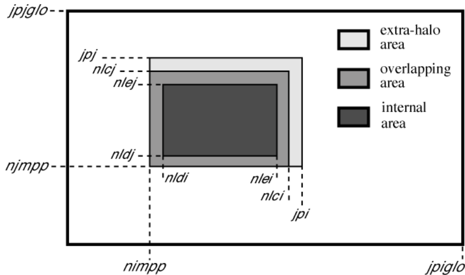
FIGURE 8.5 – Positioning of a sub-domain when massively parallel processing is used.
