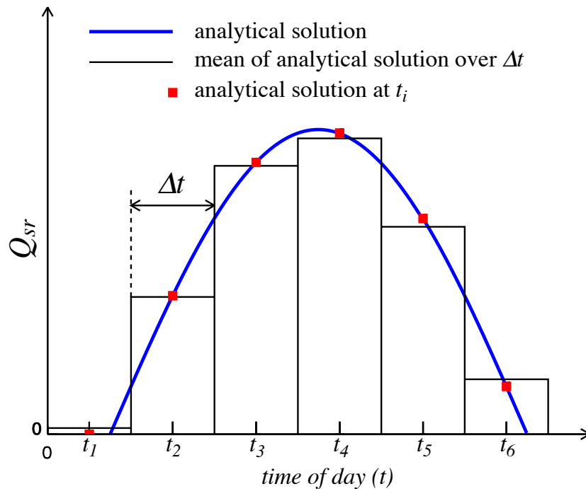
FIGURE 7.1 – Example of reconstruction of the diurnal cycle variation of short wave flux from daily mean values. The reconstructed diurnal cycle (red squares) is chosen as the mid time step value of the analytically cycle (blue line), not as the mean value of the analytical cycle over a time step (black line). The misfit is however small and without systematic bias. From ?.
