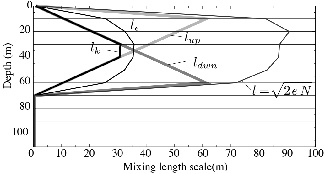
FIGURE 10.1 – Illustration of the mixing length computation.
