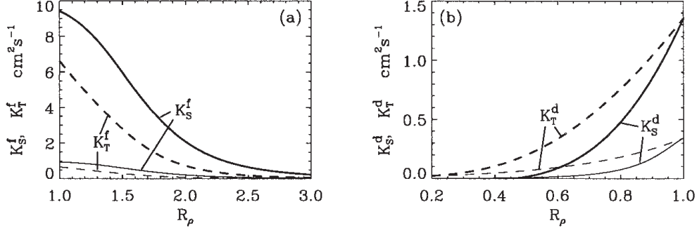
FIGURE 10.4 – From ? : (a) Diapycnal diffusivities A_f^{vT} and A_f^{vS} for temperature and salt in regions of salt fingering. Heavy curves denote A^{*v} = 10^{-3} \text{ m}^2 \cdot \text{s}^{-1} and thin curves A^{*v} = 10^{-4} \text{ m}^2 \cdot \text{s}^{-1} ; (b) diapycnal diffusivities A_d^{vT} and A_d^{vS} for temperature and salt in regions of diffusive convection. Heavy curves denote the Federov parameterisation and thin curves the Kelley parameterisation. The latter is not implemented in NEMO .
