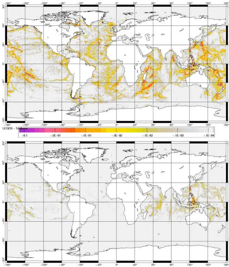
FIGURE 10.5 – (a) M2 and (b) K2 internal wave drag energy from ? ( W/m^2 ).
