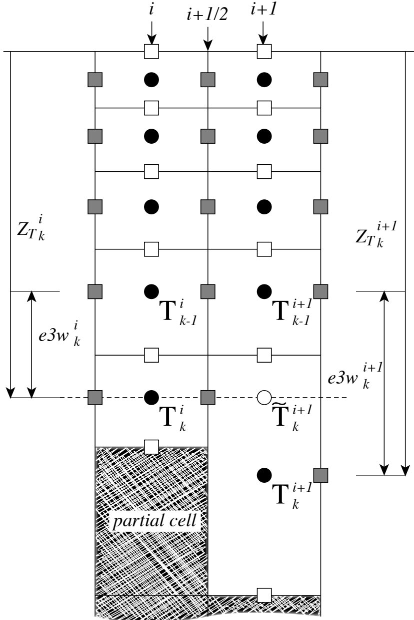
FIGURE 5.5 – Discretisation of the horizontal difference and average of tracers in the z -partial step coordinate ( ln\_zps=true ) in the case (e3w_k^{i+1} - e3w_k^i) > 0 . A linear interpolation is used to estimate \tilde{T}_k^{i+1} , the tracer value at the depth of the shallower tracer point of the two adjacent bottom T -points. The horizontal difference is then given by : \delta_{i+1/2}T_k = \tilde{T}_k^{i+1} - T_k^i and the average by : \bar{T}_k^{i+1/2} = (\tilde{T}_k^{i+1/2} - T_k^i)/2 .
