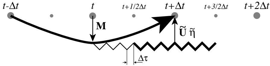
FIGURE 6.2 – Schematic of the split-explicit time stepping scheme for the external and internal modes. Time increases to the right. Internal mode time steps (which are also the model time steps) are denoted by t - \Delta t , t , t + \Delta t , and t + 2\Delta t . The curved line represents a leap-frog time step, and the smaller time steps N\Delta t_e = \frac{3}{2}\Delta t are denoted by the zig-zag line. The vertically integrated forcing \mathbf{M}(t) computed at the model time step t represents the interaction between the external and internal motions. While keeping \mathbf{M} and freshwater forcing field fixed, a leap-frog integration carries the external mode variables (surface height and vertically integrated velocity) from t to t + \frac{3}{2}\Delta t using N external time steps of length \Delta t_e . Time averaging the external fields over the \frac{2}{3}N + 1 time steps (endpoints included) centers the vertically integrated velocity and the sea surface height at the model timestep t + \Delta t . These averaged values are used to update \mathbf{M}(t) with both the surface pressure gradient and the Coriolis force, therefore providing the t + \Delta t velocity. The model time stepping scheme can then be achieved by a baroclinic leap-frog time step that carries the surface height from t - \Delta t to t + \Delta t .
