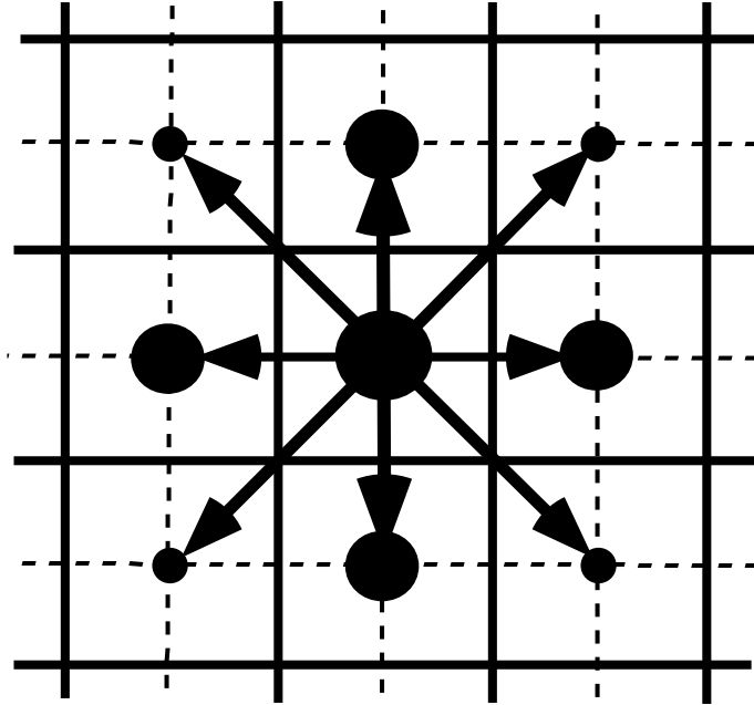
FIGURE 9.1 – averaging procedure for isopycnal slope computation.
