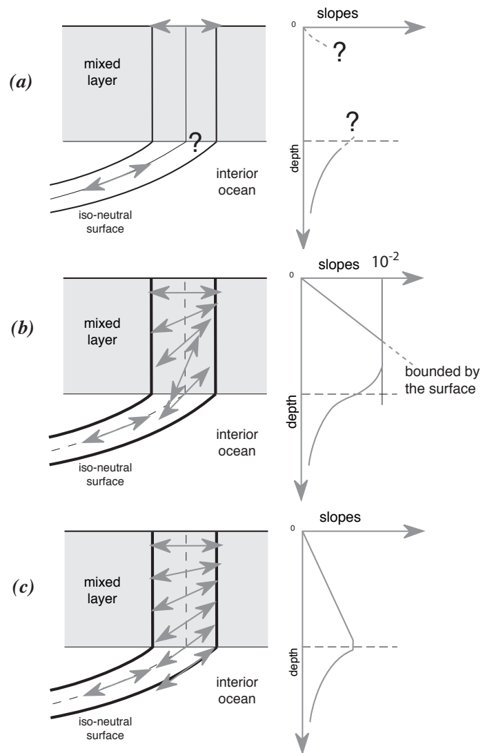
FIGURE 9.2 – Vertical profile of the slope used for lateral mixing in the mixed layer : (a) in the real ocean the slope is the iso-neutral slope in the ocean interior, which has to be adjusted at the surface boundary (i.e. it must tend to zero at the surface since there is no mixing across the air-sea interface : wall boundary condition). Nevertheless, the profile between the surface zero value and the interior iso-neutral one is unknown, and especially the value at the base of the mixed layer ; (b) profile of slope using a linear tapering of the slope near the surface and imposing a maximum slope of 1/100 ; (c) profile of slope actually used in NEMO : a linear decrease of the slope from zero at the surface to its ocean interior value computed just below the mixed layer. Note the huge change in the slope at the base of the mixed layer between (b) and (c).
