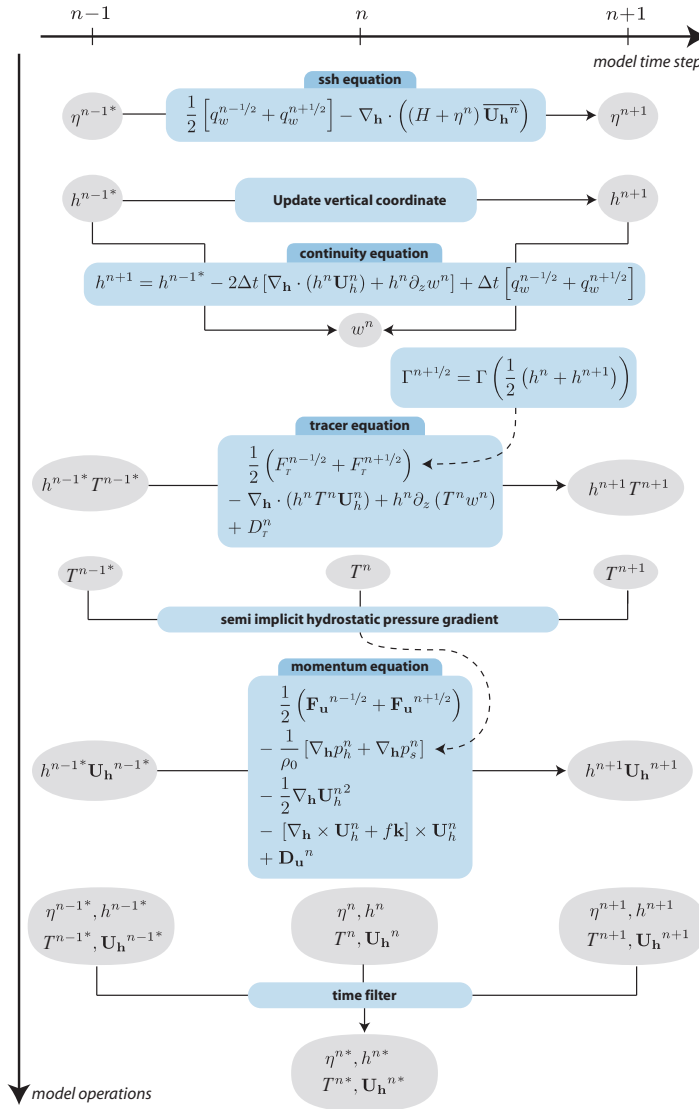
FIGURE 3.1 – Sketch of the leapfrog time stepping sequence in NEMO from ?. The use of semi-implicit computation of the hydrostatic pressure gradient requires the tracer equation to be step forward prior to the momentum equation. The need of the knowledge of the vertical scale factor (here denoted as h ) requires the sea surface height and the continuity equation to be step forward prior to the computation of the tracer equation. Note that how the surface pressure gradient \nabla p_s is evaluated is not represented here (see § 6.5).
