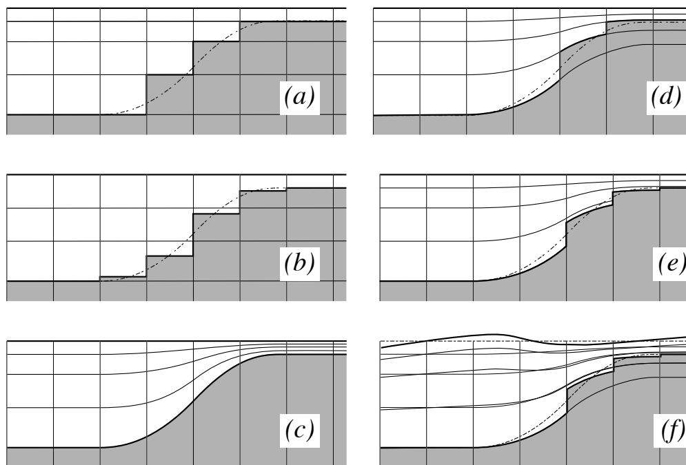
FIGURE 4.5 – The ocean bottom as seen by the model : (a) z -coordinate with full step, (b) z -coordinate with partial step, (c) s -coordinate : terrain following representation, (d) hybrid s - z coordinate, (e) hybrid s - z coordinate with partial step, and (f) same as (e) but with variable volume associated with the non-linear free surface. Note that the variable volume option ( key_vvl ) can be used with any of the 5 coordinates (a) to (e).
