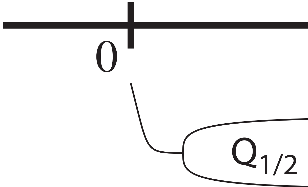
FIGURE 3.2 – Illustration of forcing integration methods. "Traditional" formulation (top) where a centred forcing is applied over a 2\Delta t period and modified formulation (bottom) where a mean forcing over the two successive time step is applied over a 2\Delta t period.
