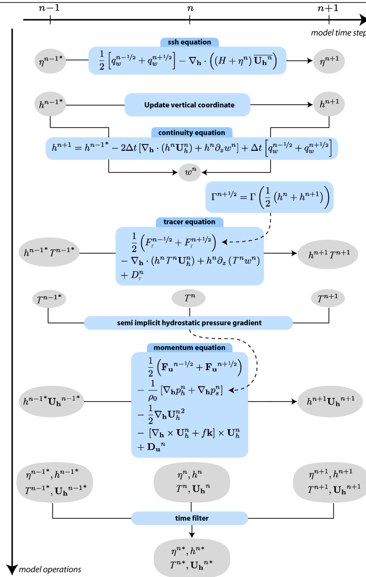
FIGURE 3.1 – Sketch of the leapfrog time stepping sequence in NEMO from ?. The use of a semi-implicit computation of the hydrostatic pressure gradient requires the tracer equation to be stepped forward prior to the momentum equation. The need for knowledge of the vertical scale factor (here denoted as h ) requires the sea surface height and the continuity equation to be stepped forward prior to the computation of the tracer equation. Note that the method for the evaluation of the surface pressure gradient \nabla p_s is not presented here (see § 6.5).
