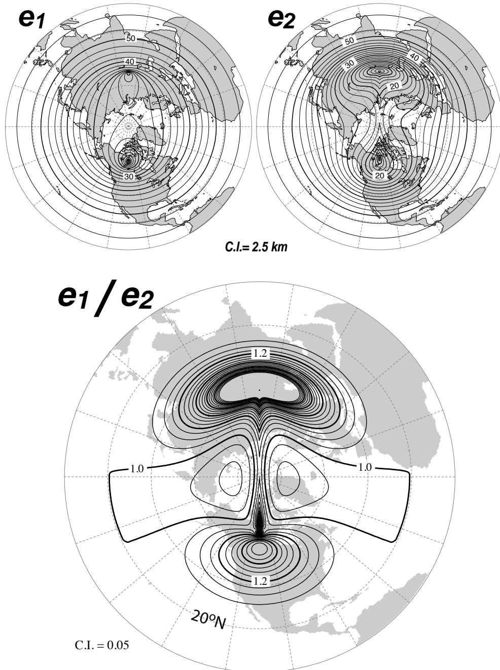
FIG. 13.5 – Top : Horizontal scale factors ( e_1 , e_2 ) and Bottom : ratio of anisotropy ( e_1/e_2 ) for ORCA 0.5^\circ mesh. South of 20^\circ N a Mercator grid is used ( e_1 = e_2 ) so that the anisotropy ratio is 1. Poleward of 20^\circ N , the two "north pole" introduce a weak anisotropy over the ocean areas ( < 1.2 ) except in vicinity of Victoria Island (Canadian Arctic Archipelago).
