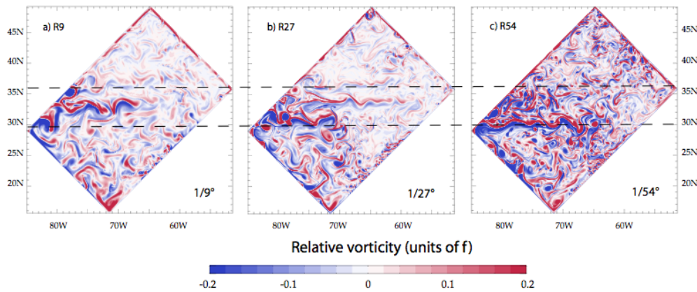
FIG. 13.6 – Snapshot of relative vorticity at the surface of the model domain in GYRE R9, R27 and R54. From Lévy et al. [2010].
