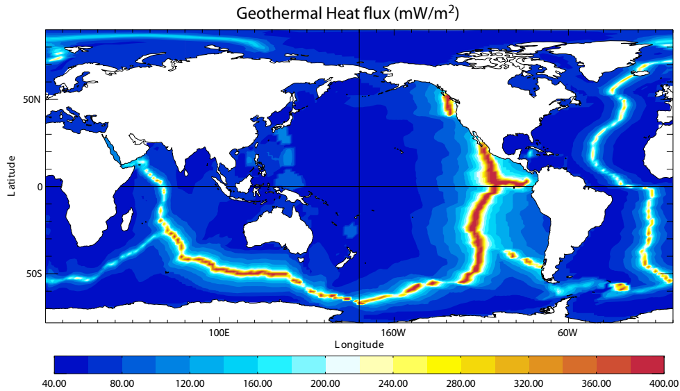
FIG. 4.2 – Geothermal Heat flux (in mW.m^{-2} ) used by Emile-Geay and Madec [2008]. It is inferred from the age of the sea floor and the formulae of Stein and Stein [1992].
