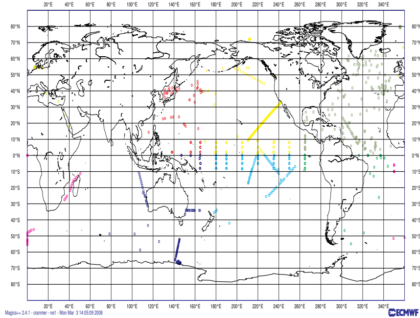
FIG. 12.1: Example of the distribution of observations with the geographical distribution of observational data.
