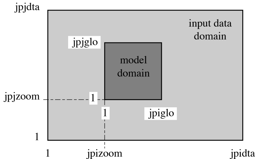
FIG. 14.2: Position of a model domain compared to the data input domain when the zoom functionality is used.
