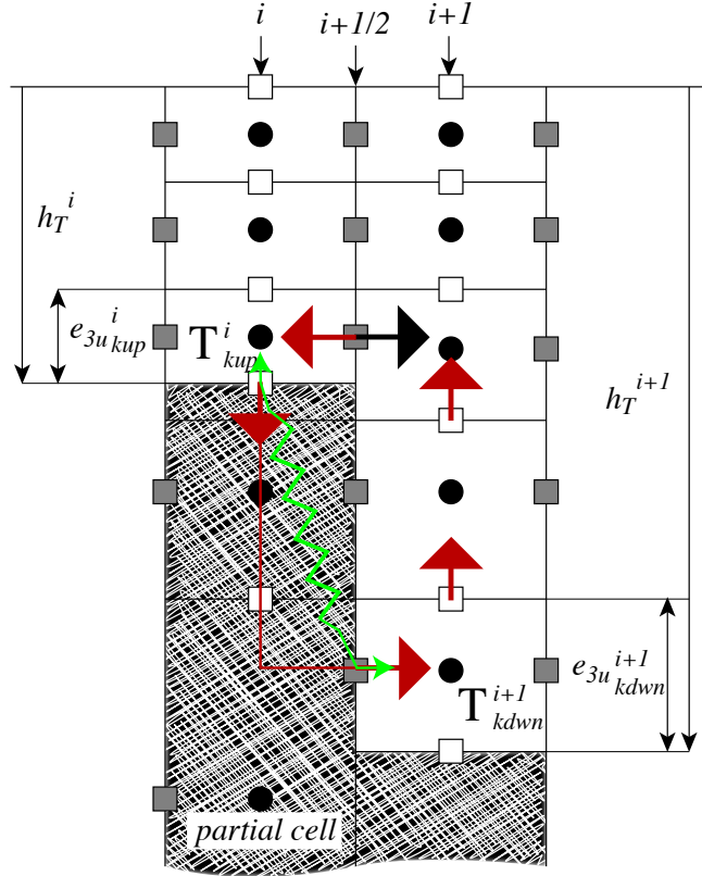
FIG. 5.4: Advective/diffusive Bottom Boundary Layer. The BBL parameterisation is activated when \rho_{kup}^i is larger than \rho_{kdown}^{i+1} . Red arrows indicate the additional overturning circulation due to the advective BBL. The transport of the downslope flow is defined either as the transport of the bottom ocean cell (black arrow), or as a function of the along slope density gradient. The green arrow indicates the diffusive BBL flux directly connecting kup and kdown ocean bottom cells. connection
