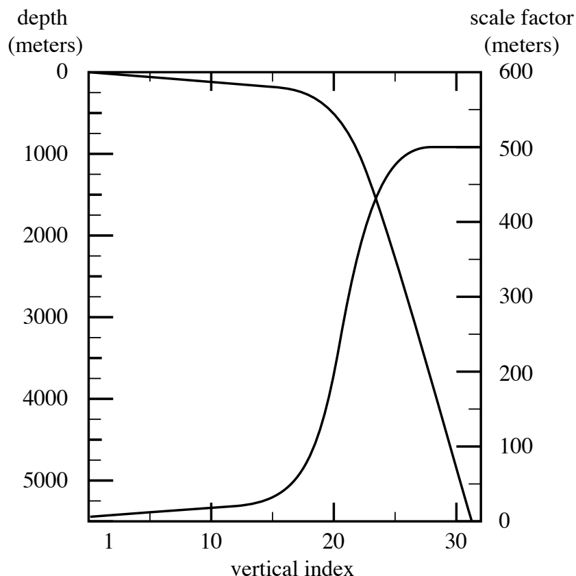
FIG. 4.6: Default vertical mesh for ORCA2 : 30 ocean levels (L30). Vertical level functions for (a) T-point depth and (b) the associated scale factor as computed from (4.13) using (4.14) in z -coordinate.
