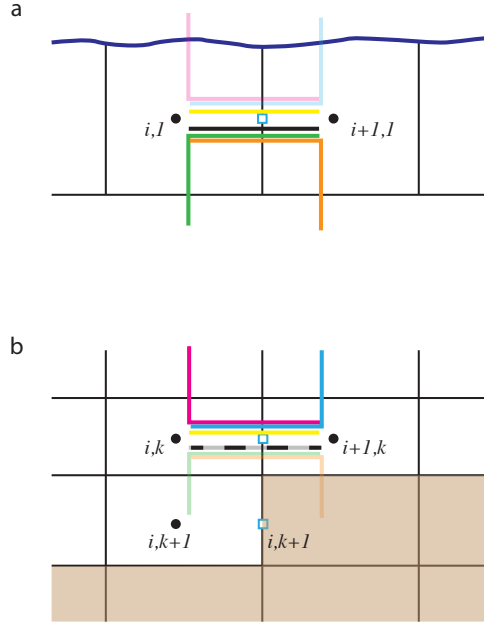
FIG. E.3: (a) Uppermost model layer k = 1 with i, 1 and i + 1, 1 tracer points (black dots), and i + 1/2, 1 u -point (blue square). Triad slopes \frac{1}{2} \mathbb{R}_{1/2}^{-1/2} (magenta) and \frac{1}{2} \mathbb{R}_{-1/2}^{-1/2} (blue) poking through the ocean surface are masked (faded in figure). However, the lateral _{11} contributions towards \frac{1}{2} \mathbb{F}_{u_{1/2}}^{-1/2} and \frac{1}{2} \mathbb{F}_{u_{-1/2}}^{-1/2} (yellow line) are still applied, giving diapycnal diffusive fluxes. (b) Both near bottom triad slopes \frac{1}{2} \mathbb{R}_{1/2}^{1/2} and \frac{1}{2} \mathbb{R}_{-1/2}^{1/2} are masked when either of the i, k + 1 or i + 1, k + 1 tracer points is masked, i.e. the i, k + 1 u -point is masked. The associated lateral fluxes (grey-black dashed line) are masked if ln_botmix_grif=.false. , but left unmasked, giving bottom mixing, if ln_botmix_grif=.true.
