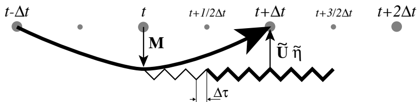
FIGURE 6.2: Schematic of the split-explicit time stepping scheme for the external and internal modes. Time increases to the right. Internal mode time steps (which are also the model time steps) are denoted by t - \Delta t , t , t + \Delta t , and t + 2\Delta t . The curved line represents a leap-frog time step, and the smaller time steps N\Delta t_e = \frac{3}{2}\Delta t are denoted by the zig-zag line. The vertically integrated forcing \mathbf{M}(t) computed at the model time step t represents the interaction between the external and internal motions. While keeping \mathbf{M} and freshwater forcing field fixed, a leap-frog integration carries the external mode variables (surface height and vertically integrated velocity) from t to t + \frac{3}{2}\Delta t using N external time steps of length \Delta t_e . Time averaging the external fields over the \frac{2}{3}N + 1 time steps (endpoints included) centers the vertically integrated velocity and the sea surface height at the model timestep t + \Delta t . These averaged values are used to update \mathbf{M}(t) with both the surface pressure gradient and the Coriolis force, therefore providing the t + \Delta t velocity. The model time stepping scheme can then be achieved by a baroclinic leap-frog time step that carries the surface height from t - \Delta t to t + \Delta t .
