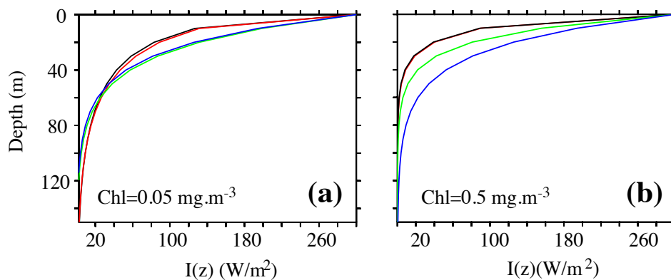
FIGURE 5.2: Penetration profile of the downward solar irradiance calculated by four models. Two waveband chlorophyll-independent formulation (blue), a chlorophyll-dependent monochromatic formulation (green), 4 waveband RGB formulation (red), 61 waveband Morel (1988) formulation (black) for a chlorophyll concentration of (a) \text{Chl}=0.05 \text{ mg.m}^{-3} and (b) \text{Chl}=0.5 \text{ mg.m}^{-3} . From ?.
