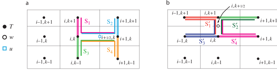
FIGURE E.1: (a) Arrangement of triads S_i and tracer gradients to give lateral tracer flux from box i, k to i + 1, k (b) Triads S'_i and tracer gradients to give vertical tracer flux from box i, k to i, k + 1 .
