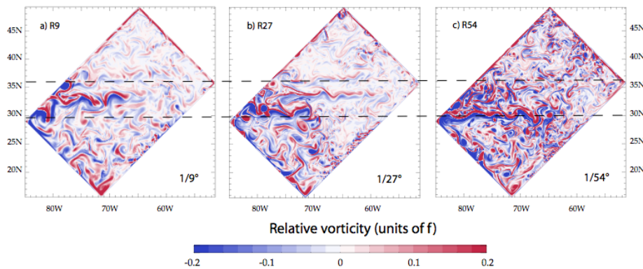
FIGURE 15.3: Snapshot of relative vorticity at the surface of the model domain in GYRE R9, R27 and R54. From ?.
