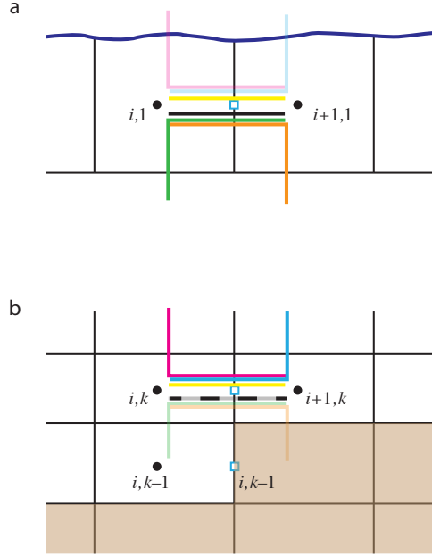
FIGURE E.3: (a) Uppermost model layer k = 1 with i, 1 and i + 1, 1 tracer points (black dots), and i + 1/2, 1 u -point (blue square). Triad slopes \frac{1}{i}\mathbb{R}_{1/2}^{-1/2} (magenta) and \frac{1}{i+1}\mathbb{R}_{-1/2}^{-1/2} (blue) poking through the ocean surface are masked (faded in figure). However, the lateral _{11} contributions towards \frac{1}{i}\mathbb{F}_{u1/2}^{-1/2} and \frac{1}{i+1}\mathbb{F}_{u-1/2}^{-1/2} (yellow line) are still applied, giving diapycnal diffusive fluxes. (b) Both near bottom triad slopes \frac{k}{i}\mathbb{R}_{1/2}^{1/2} and \frac{k}{i+1}\mathbb{R}_{-1/2}^{1/2} are masked when either of the i, k + 1 or i + 1, k + 1 tracer points is masked, i.e. the i, k + 1 u -point is masked. The associated lateral fluxes (grey-black dashed line) are masked if botmix_grif=false. , but left unmasked, giving bottom mixing, if botmix_grif=true.
