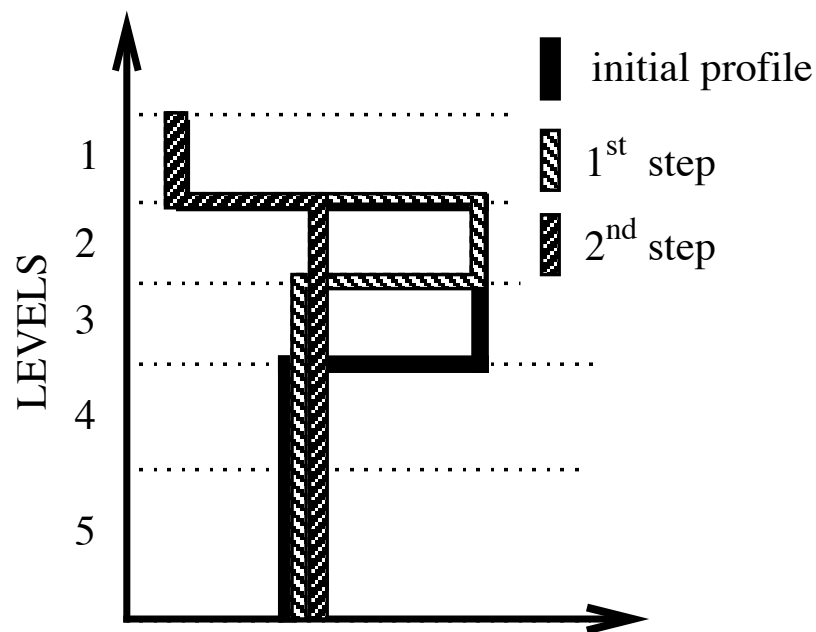
FIGURE 10.3: Example of an unstable density profile treated by the non penetrative convective adjustment algorithm. 1 st step : the initial profile is checked from the surface to the bottom. It is found to be unstable between levels 3 and 4. They are mixed. The resulting \rho is still larger than \rho(5) : levels 3 to 5 are mixed. The resulting \rho is still larger than \rho(6) : levels 3 to 6 are mixed. The 1 st step ends since the density profile is then stable below the level 3. 2 nd step : the new \rho profile is checked following the same procedure as in 1 st step : levels 2 to 5 are mixed. The new density profile is checked. It is found stable : end of algorithm.
