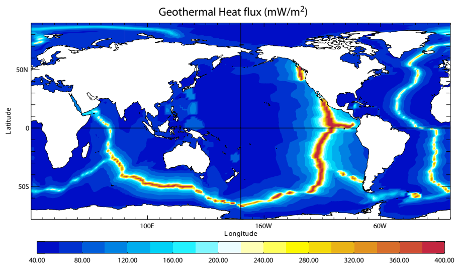
FIGURE 5.3: Geothermal Heat flux (in mW.m^{-2} ) used by ?. It is inferred from the age of the sea floor and the formulae of ?.
