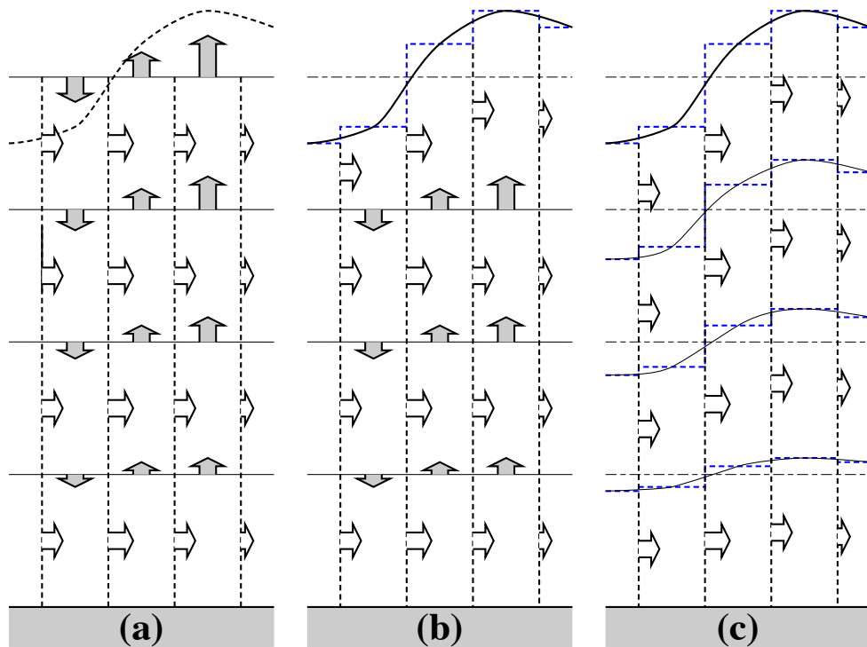
FIGURE 2.3 – (a) z -coordinate in linear free-surface case ; (b) z -coordinate in non-linear free surface case ; (c) re-scaled height coordinate (become popular as the z^* -coordinate [Adcroft and Campin 2004] ).
