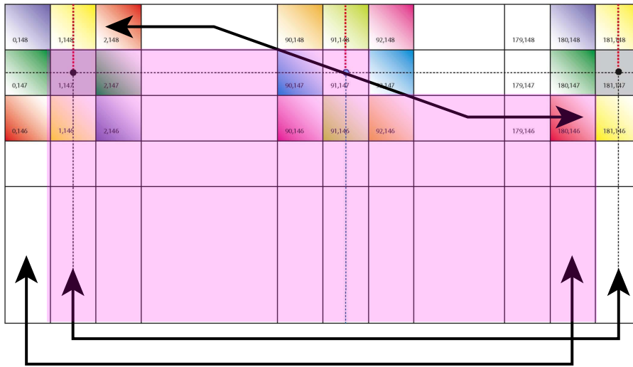
FIGURE 8.4 – North fold boundary with a T -point pivot and cyclic east-west boundary condition ( j_{\text{perio}} = 4 ), as used in ORCA 2, 1/4, and 1/12. Pink shaded area corresponds to the inner domain mask (see text).
