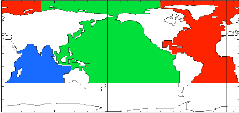
FIGURE 11.1 – Decomposition of the World Ocean (here ORCA2) into sub-basin used in to compute the heat and salt transports as well as the meridional stream-function : Atlantic basin (red), Pacific basin (green), Indian basin (bleue), Indo-Pacific basin (bleue+green). Note that semi-enclosed seas (Red, Med and Baltic seas) as well as Hudson Bay are removed from the sub-basins. Note also that the Arctic Ocean has been split into Atlantic and Pacific basins along the North fold line.
