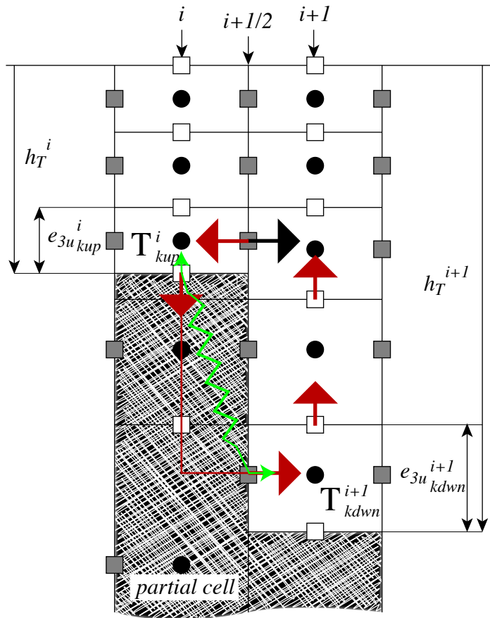
FIGURE 5.4 – Advective/diffusive Bottom Boundary Layer. The BBL parameterisation is activated when \rho_{kup}^i is larger than \rho_{kdwn}^{i+1} . Red arrows indicate the additional overturning circulation due to the advective BBL. The transport of the downslope flow is defined either as the transport of the bottom ocean cell (black arrow), or as a function of the along slope density gradient. The green arrow indicates the diffusive BBL flux directly connecting kup and kdwn ocean bottom cells. connection
