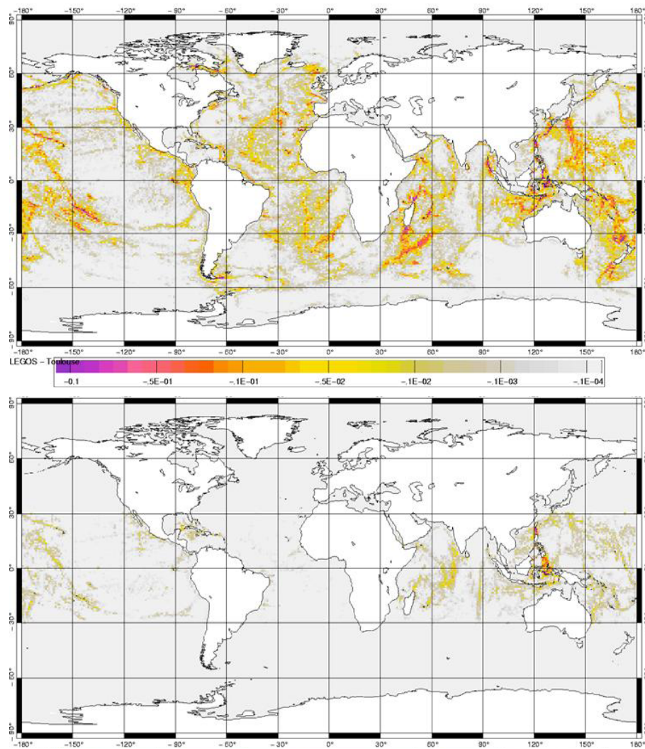
FIGURE 10.5 – (a) M2 and (b) K2 internal wave drag energy from Carrère and Lyard [2003] ( W/m^2 ).
