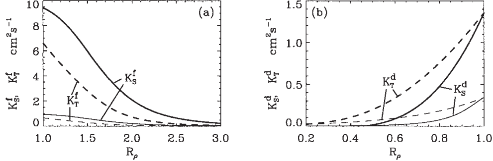
FIGURE 10.4 – From Merryfield et al. [1999] : (a) Diapycnal diffusivities A_f^{vT} and A_f^{vS} for temperature and salt in regions of salt fingering. Heavy curves denote A^{*v} = 10^{-3} \text{ m}^2 \cdot \text{s}^{-1} and thin curves A^{*v} = 10^{-4} \text{ m}^2 \cdot \text{s}^{-1} ; (b) diapycnal diffusivities A_d^{vT} and A_d^{vS} for temperature and salt in regions of diffusive convection. Heavy curves denote the Federov parameterisation and thin curves the Kelley parameterisation. The latter is not implemented in NEMO .
