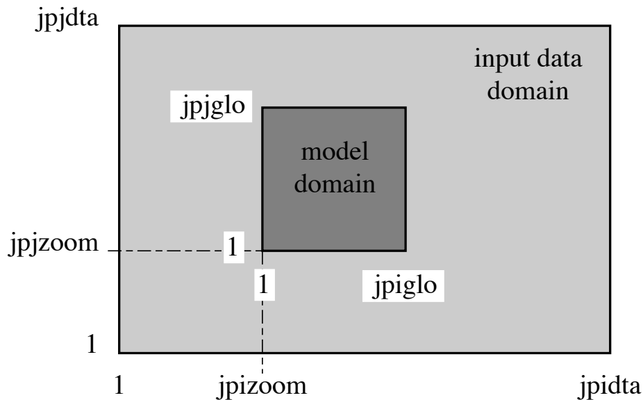
FIG. 13.2 – Position of a model domain compared to the data input domain when the zoom functionality is used.
