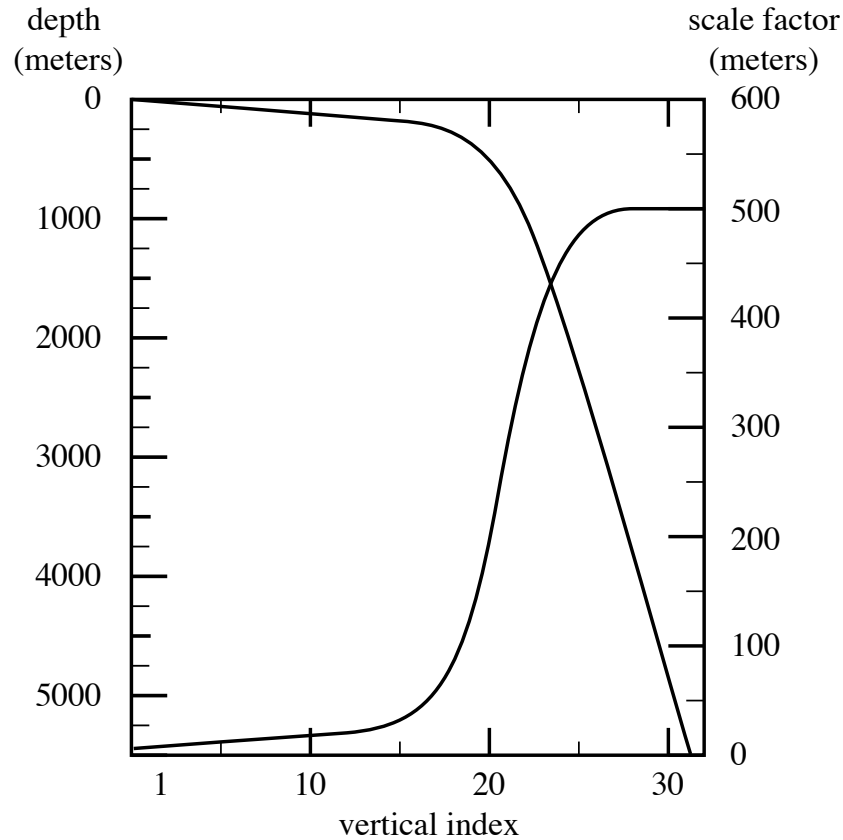
FIGURE 4.6: Default vertical mesh for ORCA2 : 30 ocean levels (L30). Vertical level functions for (a) T-point depth and (b) the associated scale factor as computed from (??) using (??) in z -coordinate.
