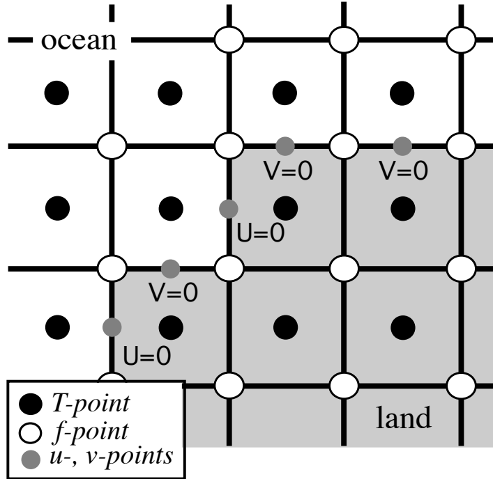
Figure 8.1: Lateral boundary (thick line) at T-level. The velocity normal to the boundary is set to zero.
