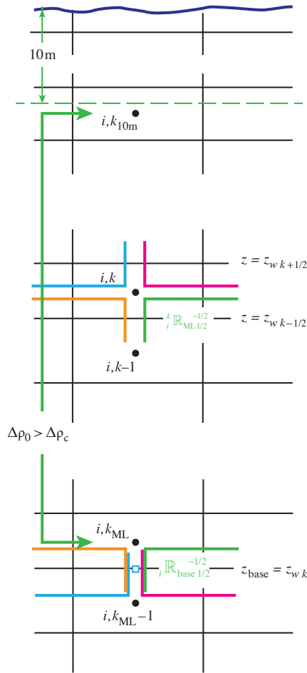
Figure E.4: Definition of mixed-layer depth and calculation of linearly tapered triads. The figure shows a water column at a given i, j (simplified to i ), with the ocean surface at the top. Tracer points are denoted by bullets, and black lines the edges of the tracer cells; k increases upwards.
