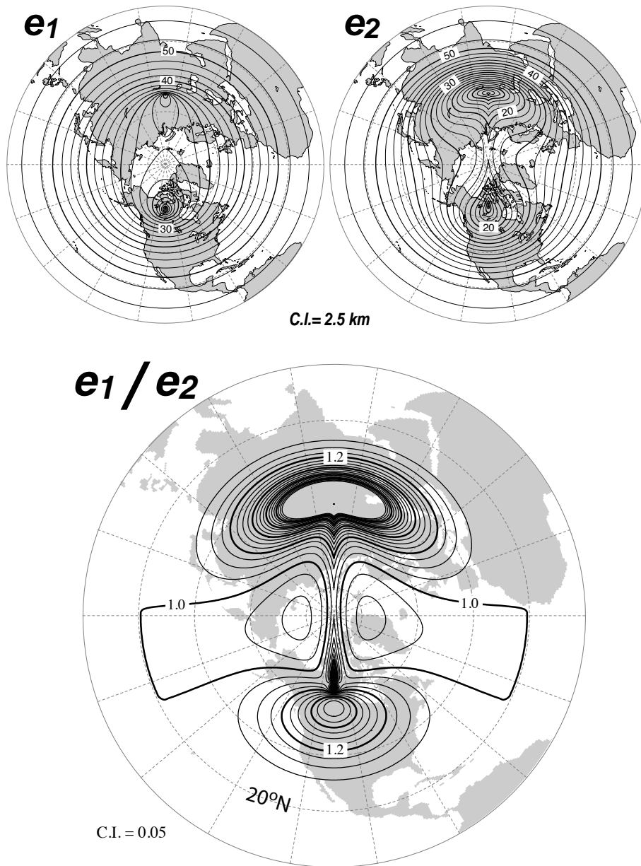
Figure 15.2: Top: Horizontal scale factors ( e_1 , e_2 ) and Bottom: ratio of anisotropy ( e_1/e_2 ) for ORCA 0.5 mesh. South of 20N a Mercator grid is used ( e_1 = e_2 ) so that the anisotropy ratio is 1. Poleward of 20N, the two "north pole" introduce a weak anisotropy over the ocean areas ( < 1.2 ) except in vicinity of Victoria Island (Canadian Arctic Archipelago).
