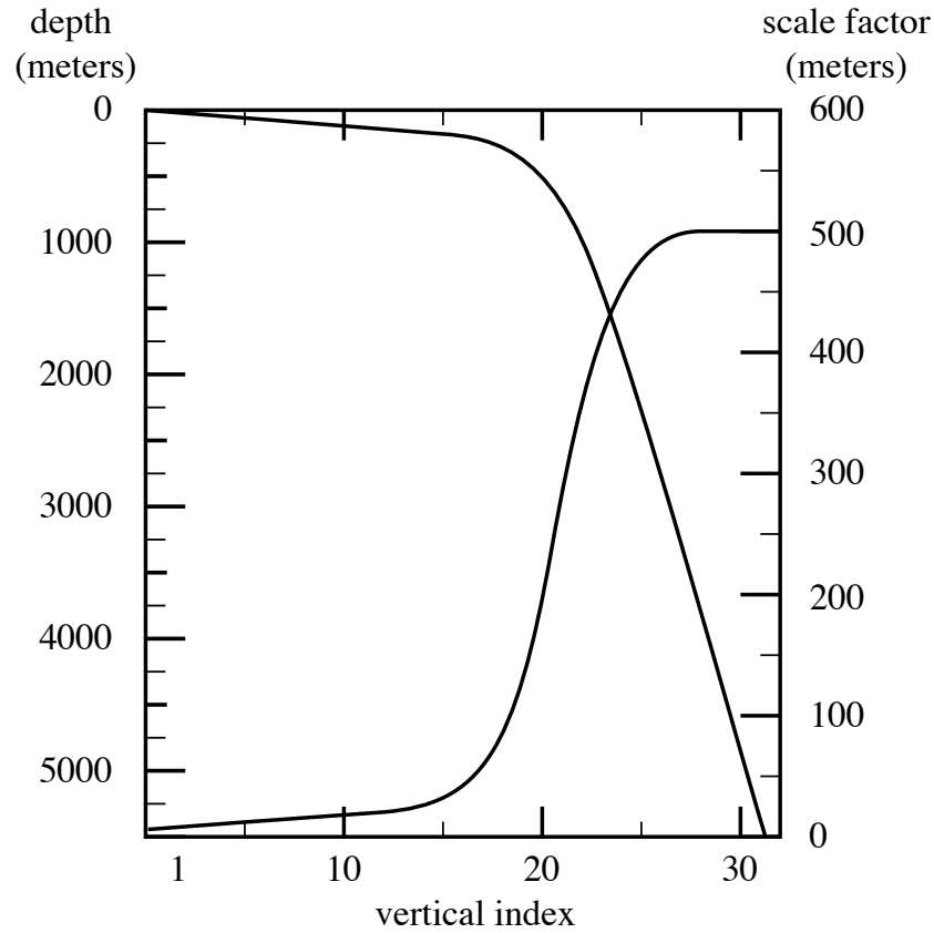
Figure 4.6: Default vertical mesh for ORCA2: 30 ocean levels (L30). Vertical level functions for (a) T-point depth and (b) the associated scale factor as computed from (4.13) using (4.14) in z -coordinate.
