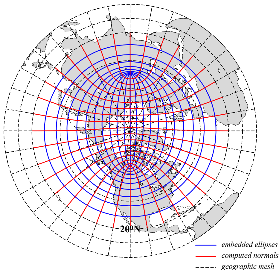
Figure 15.1: ORCA mesh conception. The departure from an isotropic Mercator grid start poleward of 20N. The two "north pole" are the foci of a series of embedded ellipses (blue curves) which are determined analytically and form the i-lines of the ORCA mesh (pseudo latitudes). Then, following Madec and Imbard [1996] , the normal to the series of ellipses (red curves) is computed which provide the j-lines of the mesh (pseudo longitudes).
