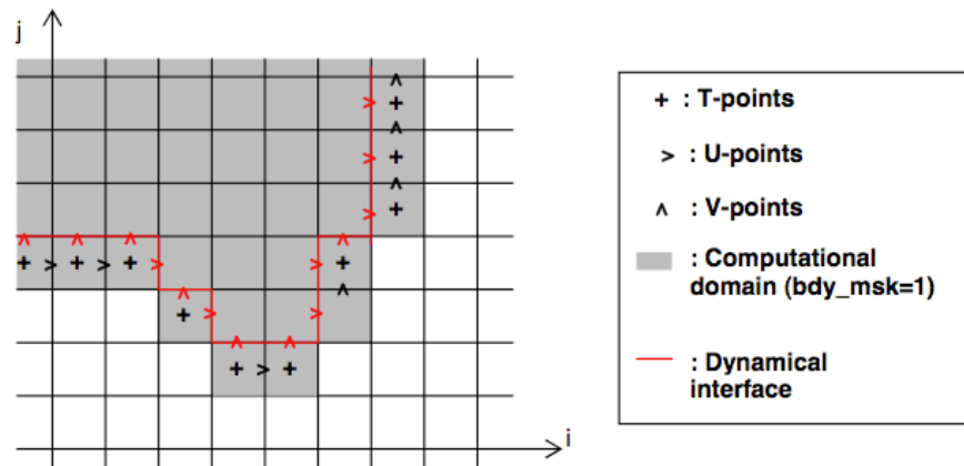
FIGURE 8.8: Example of geometry of unstructured open boundary
