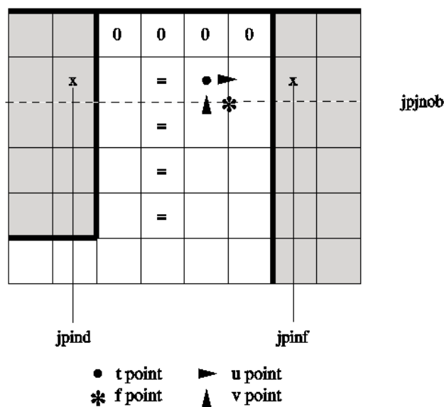
FIGURE 8.7: Localization of the North open boundary points.
