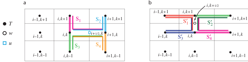
FIGURE E.1: (a) Arrangement of triads S_i and tracer gradients to give lateral tracer flux from box i, k to i + 1, k (b) Triads S'_i and tracer gradients to give vertical tracer flux from box i, k to i, k + 1 .
