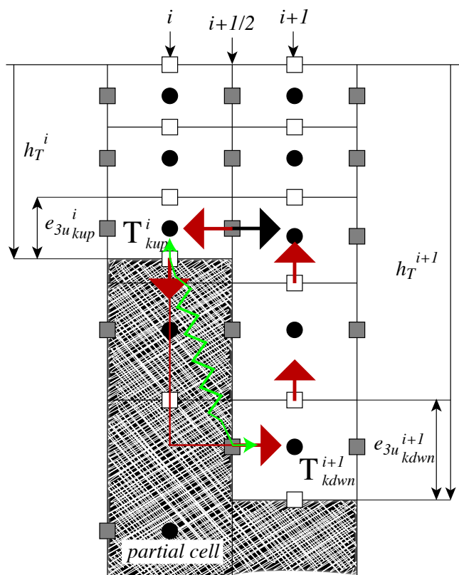
FIGURE 5.4: Advective/diffusive Bottom Boundary Layer. The BBL parameterisation is activated when \rho_{kup}^i is larger than \rho_{kdown}^{i+1} . Red arrows indicate the additional overturning circulation due to the advective BBL. The transport of the downslope flow is defined either as the transport of the bottom ocean cell (black arrow), or as a function of the along slope density gradient. The green arrow indicates the diffusive BBL flux directly connecting kup and kdown ocean bottom cells. connection
