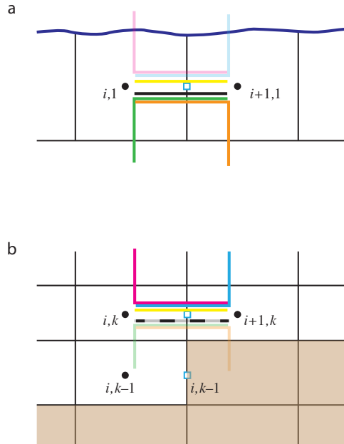
FIGURE E.3: (a) Uppermost model layer k = 1 with i, 1 and i + 1, 1 tracer points (black dots), and i + 1/2, 1 u -point (blue square). Triad slopes ^1\mathbb{R}_{1/2}^{-1/2} (magenta) and ^1_{i+1}\mathbb{R}_{-1/2}^{-1/2} (blue) poking through the ocean surface are masked (faded in figure).
