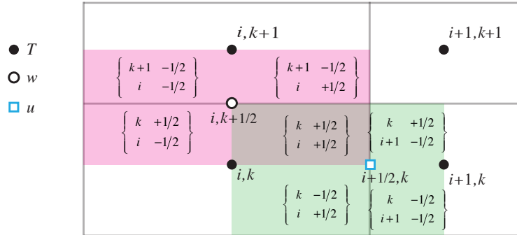
FIGURE E.2: Triad notation for quarter cells. T -cells are inside boxes, while the i + \frac{1}{2}, k u -cell is shaded in green and the i, k + \frac{1}{2} w -cell is shaded in pink.
