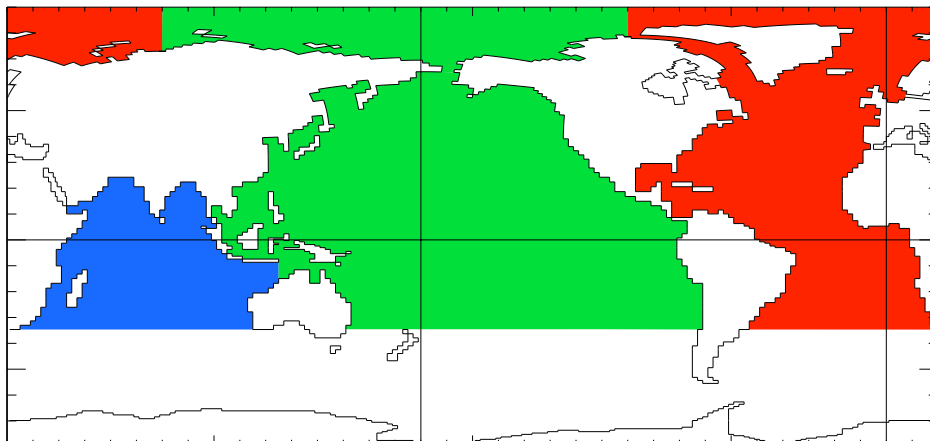
FIGURE 11.1: Decomposition of the World Ocean (here ORCA2) into sub-basin used in to compute the heat and salt transports as well as the meridional stream-function : Atlantic basin (red), Pacific basin (green), Indian basin (bleue), Indo-Pacific basin (bleue+green). Note that semi-enclosed seas (Red, Med and Baltic seas) as well as Hudson Bay are removed from the sub-basins. Note also that the Arctic Ocean has been split into Atlantic and Pacific basins along the North fold line.
