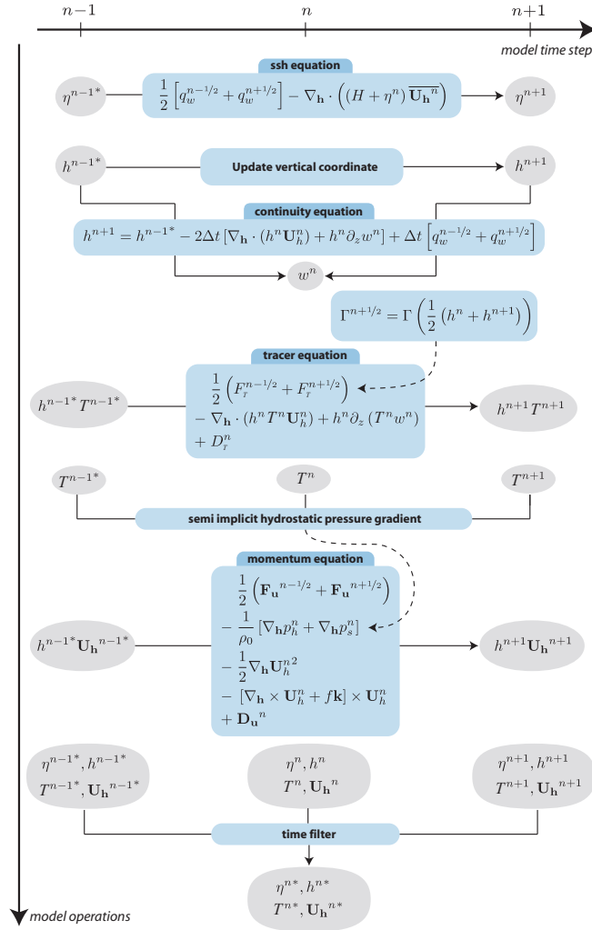
FIG. 3.1: Sketch of the leapfrog time stepping sequence in NEMO from Leclair and Madec [2009] . The use of a semi-implicit computation of the hydrostatic pressure gradient requires the tracer equation to be stepped forward prior to the momentum equation. The need for knowledge of the vertical scale factor (here denoted as h ) requires the sea surface height and the continuity equation to be stepped forward prior to the computation of the tracer equation. Note that the method for the evaluation of the surface pressure gradient \nabla p_s is not presented here (see § 6.5).
