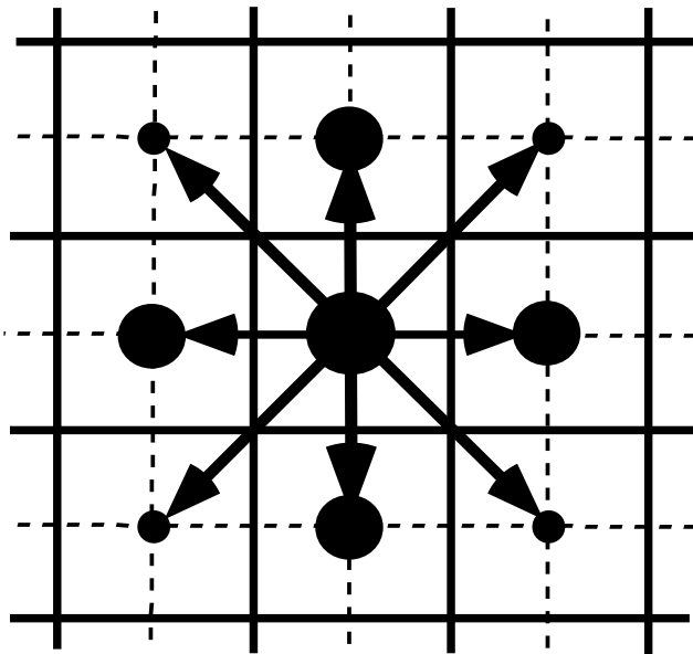
FIG. 9.1: averaging procedure for isopycnal slope computation.
