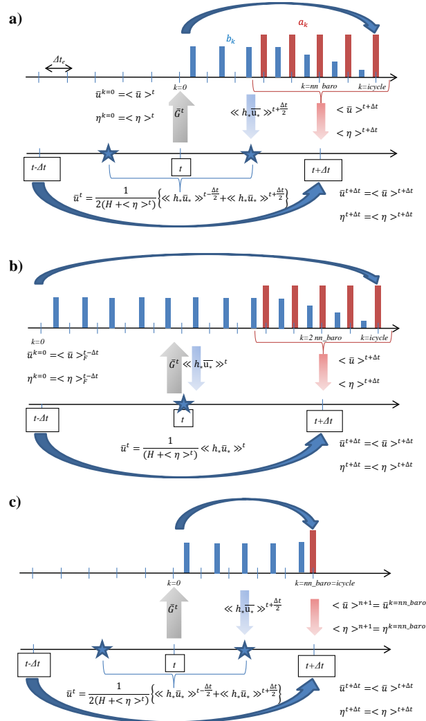
FIG. 6.2: Schematic of the split-explicit time stepping scheme for the external and internal modes. Time increases to the right. In this particular example, a box-car averaging window over nn\_baro barotropic time steps is used ( nn\_bt\_filt = 1 ) and nn\_baro = 5 . Internal mode time steps (which are also the model time steps) are denoted by t - \Delta t , t and t + \Delta t . Variables with k superscript refer to instantaneous barotropic variables, \langle \rangle and \ll \rangle \gg operator refer to time filtered variables using respectively primary (red vertical bars) and secondary weights (blue vertical bars). The former are used to obtain time filtered quantities at t + \Delta t while the latter are used to obtain time averaged transports to advect tracers. a) Forward time integration : ln\_bt\_fw=true , ln\_bt\_ave=true . b) Centred time integration : ln\_bt\_fw=false , ln\_bt\_ave=true . c) Forward time integration with no time filtering (POM-like scheme) : ln\_bt\_fw=true , ln\_bt\_ave=false .
