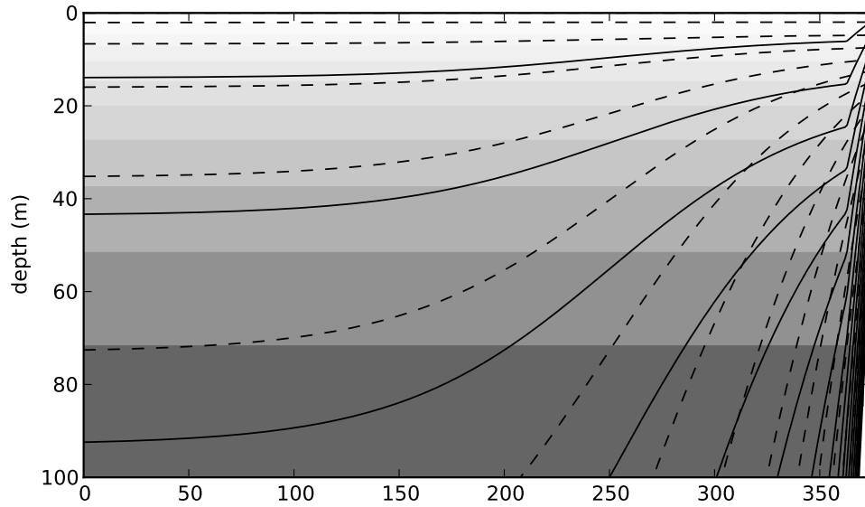
FIG. 4.8: A comparison of the Song and Haidvogel [1994] S -coordinate (solid lines), a 50 level Z -coordinate (contoured surfaces) and the Siddorn and Furner [2012] S -coordinate (dashed lines) in the surface 100m for a idealised bathymetry that goes from 50m to 5500m depth. For clarity every third coordinate surface is shown.
