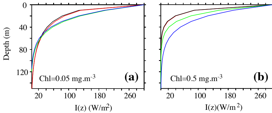
FIG. 5.2: Penetration profile of the downward solar irradiance calculated by four models. Two waveband chlorophyll-independent formulation (blue), a chlorophyll-dependent monochromatic formulation (green), 4 waveband RGB formulation (red), 61 waveband Morel (1988) formulation (black) for a chlorophyll concentration of (a) \text{Chl}=0.05 \text{ mg.m}^{-3} and (b) \text{Chl}=0.5 \text{ mg.m}^{-3} . From Lengaigne et al. [2007] .
