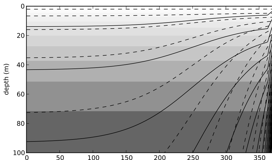
FIG. 4.8: A comparison of the \sigma_s -coordinate (solid lines), a 50 level Z -coordinate (contoured surfaces) and the \sigma_s -coordinate (dashed lines) in the surface 100m for an idealised bathymetry that goes from 50m to 5500m depth. For clarity every third coordinate surface is shown.
