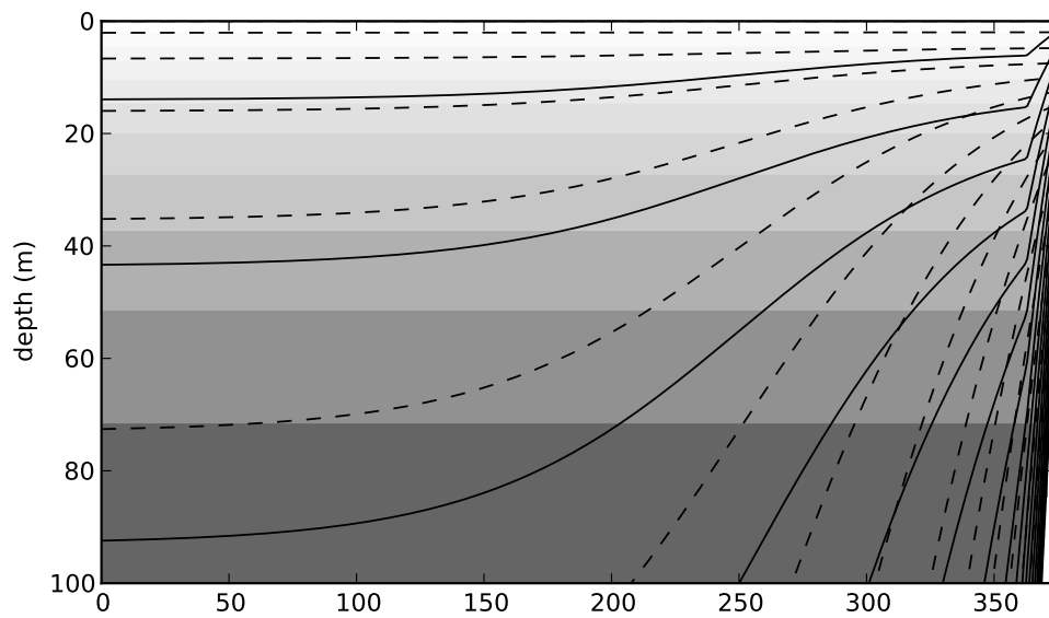
FIGURE 4.8: A comparison of the \sigma S -coordinate (solid lines), a 50 level Z -coordinate (contoured surfaces) and the \sigma S -coordinate (dashed lines) in the surface 100m for a idealised bathymetry that goes from 50m to 5500m depth. For clarity every third coordinate surface is shown.
