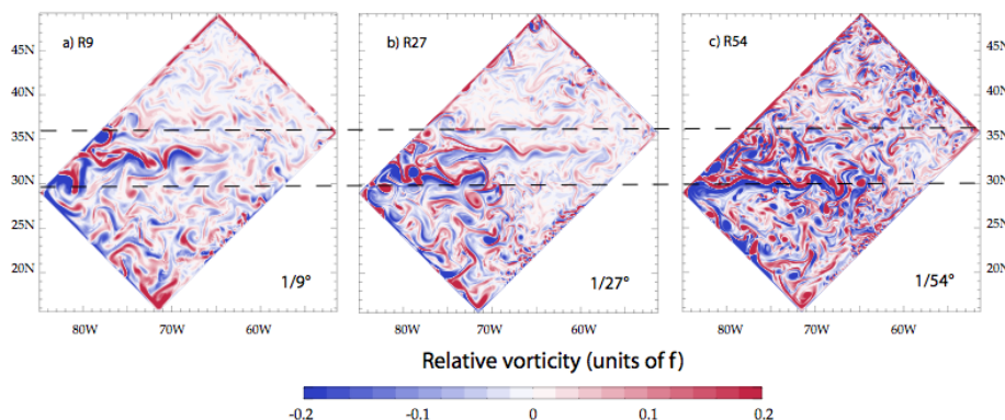
FIGURE 17.3: Snapshot of relative vorticity at the surface of the model domain in GYRE R9, R27 and R54. From Lévy et al. [2010].
