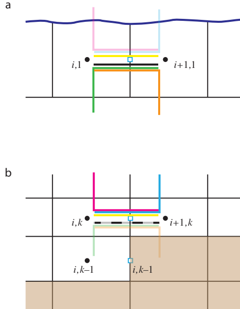
FIGURE D.3: (a) Uppermost model layer k = 1 with i, 1 and i + 1, 1 tracer points (black dots), and i + 1/2, 1 u -point (blue square). Triad slopes {}^1\mathbb{R}_{i,1/2}^{-1/2} (magenta) and {}^1\mathbb{R}_{i+1,1/2}^{-1/2} (blue) poking through the ocean surface are masked (faded in figure). However, the lateral {}_{11} contributions towards {}^1\mathbb{F}_{i,1/2}^{-1/2} and {}^1\mathbb{F}_{i+1,1/2}^{-1/2} (yellow line) are still applied, giving diapycnal diffusive fluxes. (b) Both near bottom triad slopes {}^k\mathbb{R}_{i,1/2}^{1/2} and {}^k\mathbb{R}_{i+1,1/2}^{1/2} are masked when either of the i, k + 1 or i + 1, k + 1 tracer points is masked, i.e. the i, k + 1 u -point is masked. The associated lateral fluxes (grey-black dashed line) are masked if botmix_triad=false , but left unmasked, giving bottom mixing, if botmix_triad=true .
