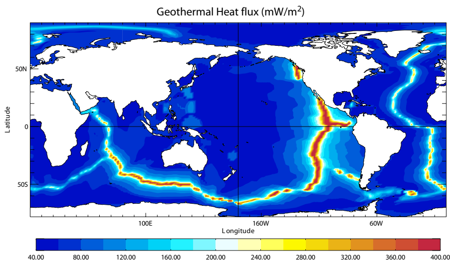
FIGURE 5.3: Geothermal Heat flux (in mW.m^{-2} ) used by Emile-Geay and Madec [2009]. It is inferred from the age of the sea floor and the formulae of Stein and Stein [1992].
