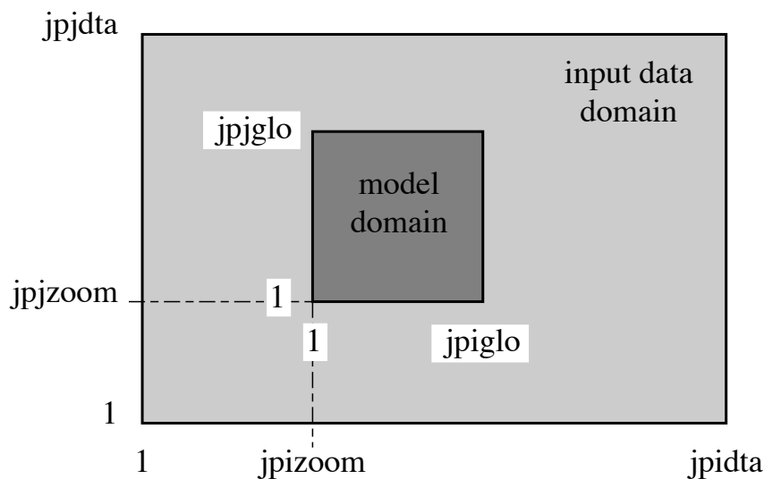
FIGURE 16.2: Position of a model domain compared to the data input domain when the zoom functionality is used.
