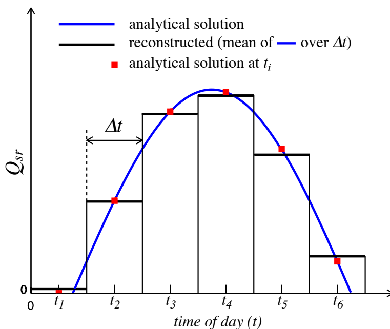
FIGURE 7.1: Example of reconstruction of the diurnal cycle variation of short wave flux from daily mean values. The reconstructed diurnal cycle (black line) is chosen as the mean value of the analytical cycle (blue line) over a time step, not as the mid time step value of the analytically cycle (red square). From Bernie et al. [2007] .
