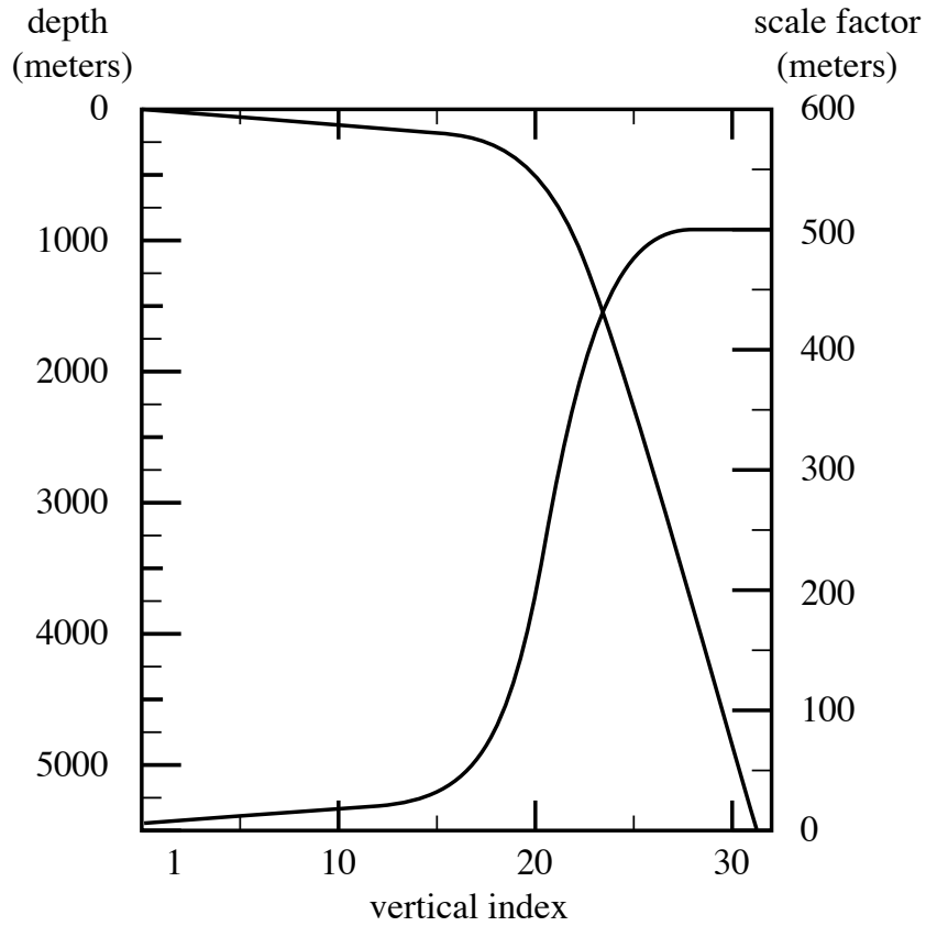
FIGURE 4.6: Default vertical mesh for ORCA2 : 30 ocean levels (L30). Vertical level functions for (a) T-point depth and (b) the associated scale factor as computed from (4.14) using (4.15) in z -coordinate.
