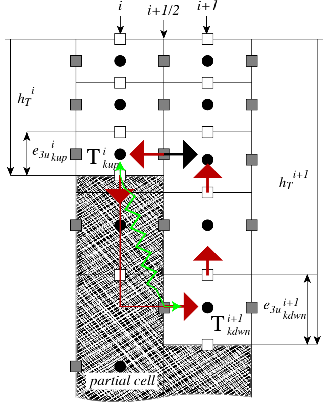
FIGURE 5.4: Advective/diffusive Bottom Boundary Layer. The BBL parameterisation is activated when \rho_{kup}^i is larger than \rho_{kdnw}^{i+1} . Red arrows indicate the additional overturning circulation due to the advective BBL. The transport of the downslope flow is defined either as the transport of the bottom ocean cell (black arrow), or as a function of the along slope density gradient. The green arrow indicates the diffusive BBL flux directly connecting kup and kdown ocean bottom cells. connection
