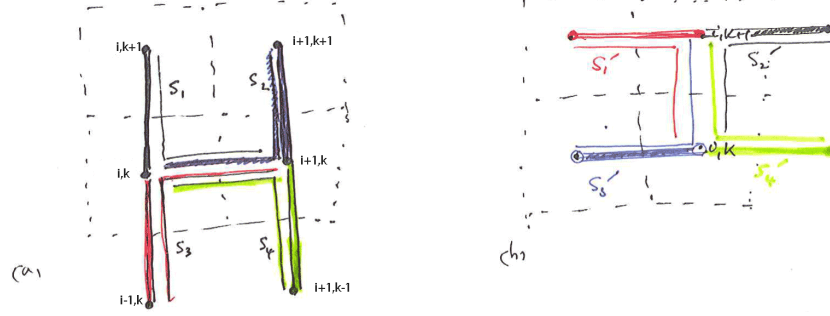
FIGURE E.1: (a) Arrangement of triads S_i and tracer gradients to give lateral tracer flux from box i, k to i + 1, k (b) Triads S'_i and tracer gradients to give vertical tracer flux from box i, k to i, k + 1 .
