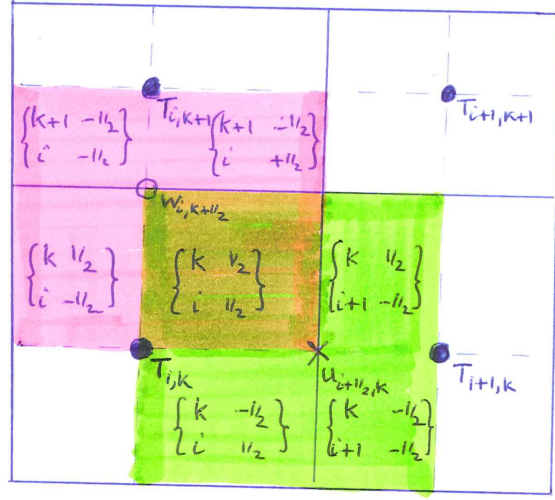
FIGURE E.2: Triad notation for quarter cells. T -cells are inside boxes, while the i + \frac{1}{2}, k u -cell is shaded in green and the i, k + \frac{1}{2} w -cell is shaded in pink.
