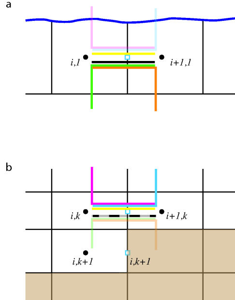
FIGURE E.3: (a) Uppermost model layer k = 1 with i, 1 and i + 1, 1 tracer points (black dots), and i + 1/2, 1 u -point (blue square). Triad slopes {}^1_i\mathbb{R}_{1/2}^{-1/2} (magenta) and {}^1_{i+1}\mathbb{R}_{-1/2}^{-1/2} (blue) poking through the ocean surface are masked (faded in figure). However, the lateral {}_{11} contributions towards {}^1_i\mathbb{F}_{u_{1/2}}^{-1/2} and {}^1_{i+1}\mathbb{F}_{u_{-1/2}}^{-1/2} (yellow line) are still applied, giving diapycnal diffusive fluxes. (b) Both near bottom triad slopes {}^k_i\mathbb{R}_{1/2}^{1/2} and {}^k_{i+1}\mathbb{R}_{-1/2}^{1/2} are masked when either of the i, k + 1 or i + 1, k + 1 tracer points is masked, i.e. the i, k + 1 u -point is masked. The associated lateral fluxes (grey-black dashed line) are masked if ln.botmix.grif=.false. , but left unmasked, giving bottom mixing, if ln.botmix.grif=.true.
