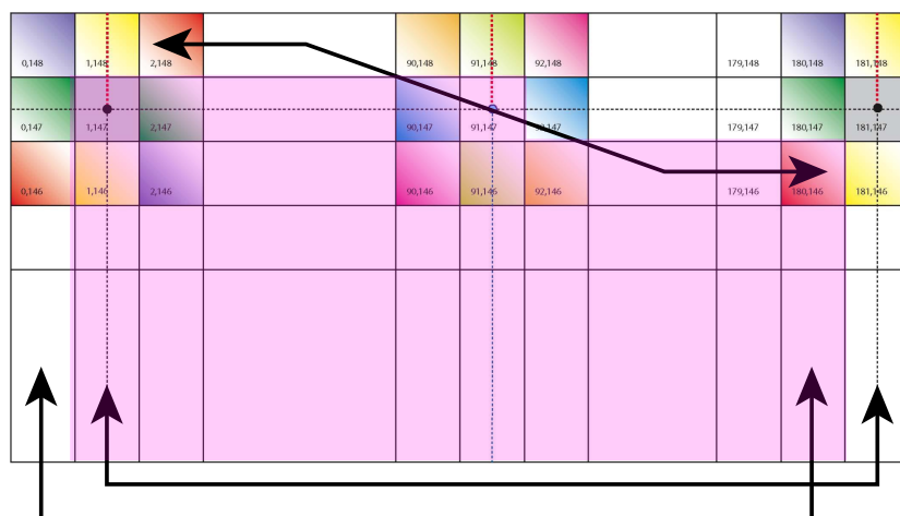
FIGURE 8.4: North fold boundary with a T -point pivot and cyclic east-west boundary condition ( j_{\text{perio}} = 4 ), as used in ORCA 2, 1/4, and 1/12. Pink shaded area corresponds to the inner domain mask (see text).
