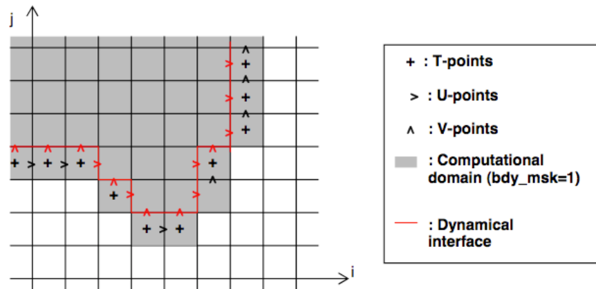
FIGURE 8.8: Example of geometry of unstructured open boundary
