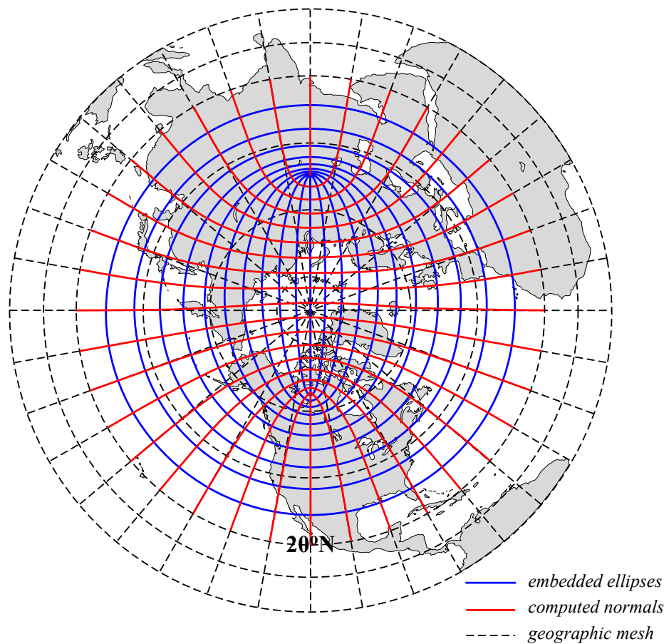
FIG. 15.1: ORCA mesh conception. The departure from an isotropic Mercator grid start poleward of 20^{\circ}\text{N} . The two "north pole" are the foci of a series of embedded ellipses (blue curves) which are determined analytically and form the i-lines of the ORCA mesh (pseudo latitudes). Then, following ?, the normal to the series of ellipses (red curves) is computed which provide the j-lines of the mesh (pseudo longitudes).
