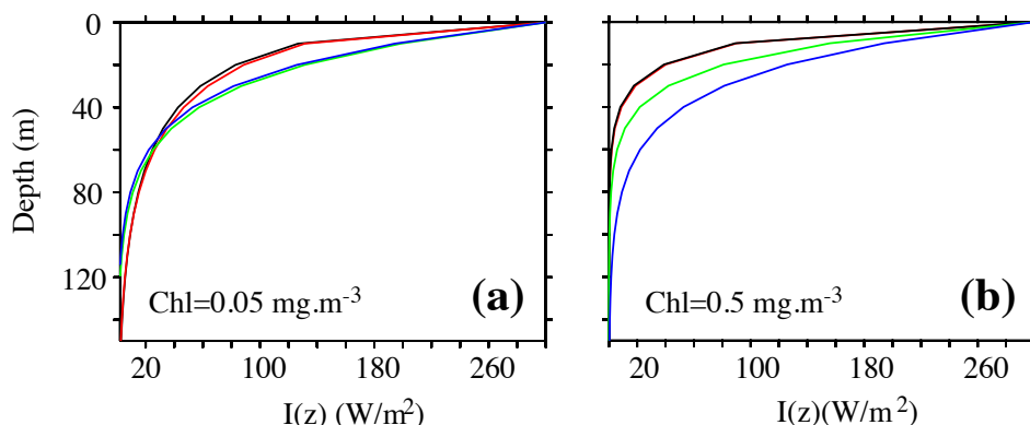
FIG. 5.2: Penetration profile of the downward solar irradiance calculated by four models. Two waveband chlorophyll-independent formulation (blue), a chlorophyll-dependent monochromatic formulation (green), 4 waveband RGB formulation (red), 61 waveband Morel (1988) formulation (black) for a chlorophyll concentration of (a) \text{Chl}=0.05 \text{ mg/m}^3 and (b) \text{Chl}=0.5 \text{ mg/m}^3 . From ?.
