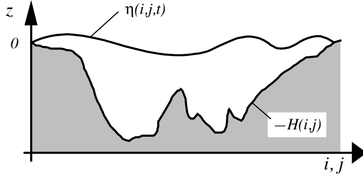
FIG. 2.1: The ocean is bounded by two surfaces, z = -H(i, j) and z = \eta(i, j, t) , where H is the depth of the sea floor and \eta the height of the sea surface. Both H and \eta are referenced to z = 0 .
