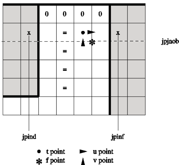
FIG. 8.7: Localization of the North open boundary points.
