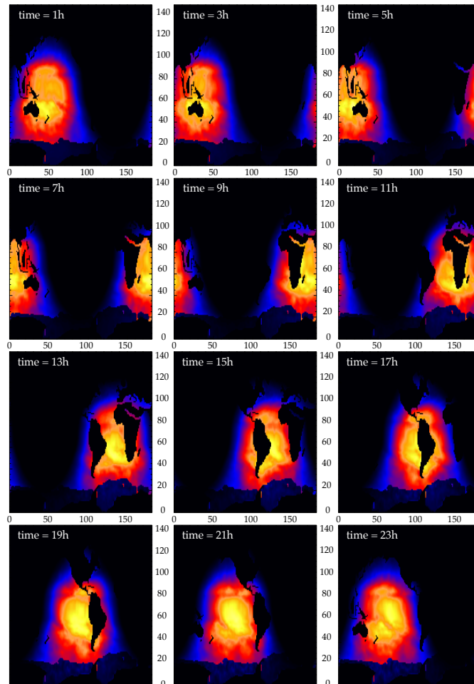
FIG. 7.2: Example of reconstruction of the diurnal cycle variation of short wave flux from daily mean values on an ORCA2 grid with a time sampling of 2 hours (from 1am to 11pm). The display is on (i,j) plane.
