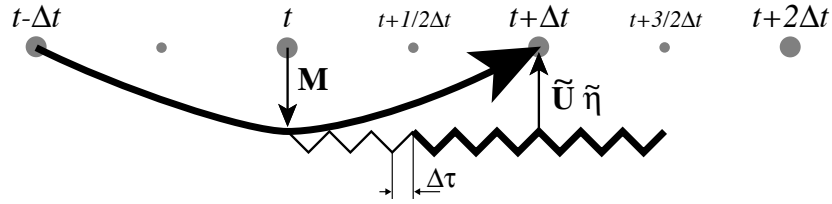
FIG. 6.2: Schematic of the split-explicit time stepping scheme for the external and internal modes. Time increases to the right. Internal mode time steps (which are also the model time steps) are denoted by t - \Delta t , t , t + \Delta t , and t + 2\Delta t . The curved line represents a leap-frog time step, and the smaller time steps N\Delta t_e = \frac{3}{2}\Delta t are denoted by the zig-zag line. The vertically integrated forcing \mathbf{M}(t) computed at the model time step t represents the interaction between the external and internal motions. While keeping \mathbf{M} and freshwater forcing field fixed, a leap-frog integration carries the external mode variables (surface height and vertically integrated velocity) from t to t + \frac{3}{2}\Delta t using N external time steps of length \Delta t_e . Time averaging the external fields over the \frac{2}{3}N + 1 time steps (endpoints included) centers the vertically integrated velocity and the sea surface height at the model timestep t + \Delta t . These averaged values are used to update \mathbf{M}(t) with both the surface pressure gradient and the Coriolis force, therefore providing the t + \Delta t velocity. The model time stepping scheme can then be achieved by a baroclinic leap-frog time step that carries the surface height from t - \Delta t to t + \Delta t .
