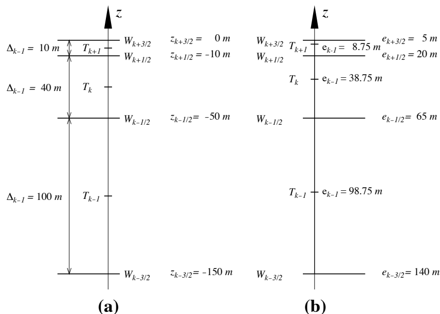
FIG. 4.4: Comparison of (a) traditional definitions of grid-point position and grid-size in the vertical, and (b) analytically derived grid-point position and scale factors. For both grids here, the same w -point depth has been chosen but in (a) the t -points are set half way between w -points while in (b) they are defined from an analytical function : z(k) = 5(i-1/2)^3 - 45(i-1/2)^2 + 140(i-1/2) - 150 . Note the resulting difference between the value of the grid-size \Delta_k and those of the scale factor e_k .
