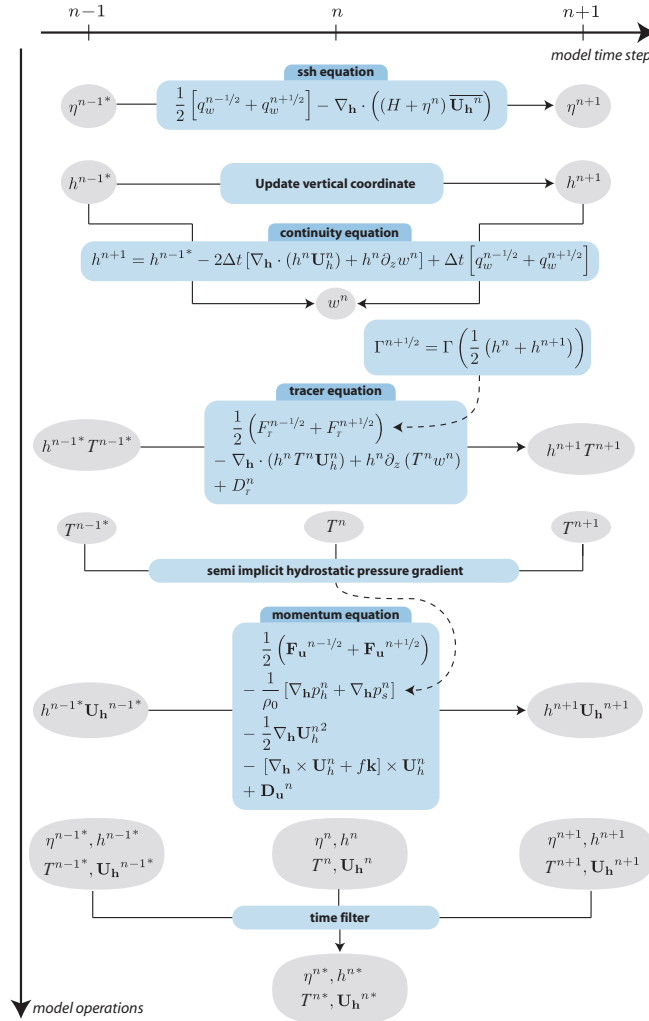
FIG. 3.1: Sketch of the leapfrog time stepping sequence in NEMO from ?. The use of a semi-implicit computation of the hydrostatic pressure gradient requires the tracer equation to be stepped forward prior to the momentum equation. The need for knowledge of the vertical scale factor (here denoted as h ) requires the sea surface height and the continuity equation to be stepped forward prior to the computation of the tracer equation. Note that the method for the evaluation of the surface pressure gradient \nabla p_s is not presented here (see § ??).
