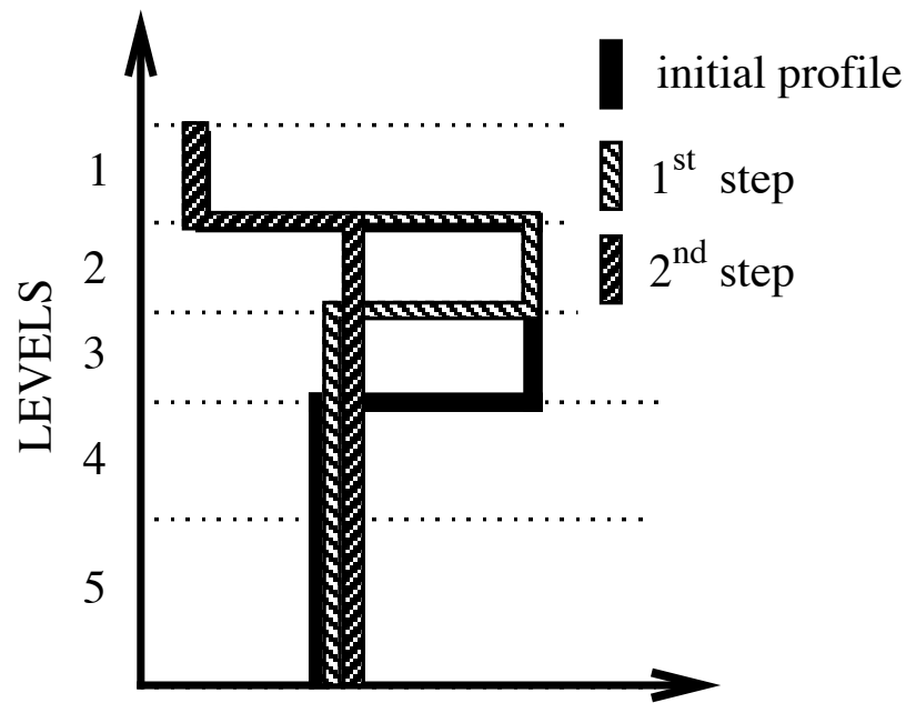
FIG. 10.3: Example of an unstable density profile treated by the non penetrative convective adjustment algorithm. 1 st step : the initial profile is checked from the surface to the bottom. It is found to be unstable between levels 3 and 4. They are mixed. The resulting \rho is still larger than \rho(5) : levels 3 to 5 are mixed. The resulting \rho is still larger than \rho(6) : levels 3 to 6 are mixed. The 1 st step ends since the density profile is then stable below the level 3. 2 nd step : the new \rho profile is checked following the same procedure as in 1 st step : levels 2 to 5 are mixed. The new density profile is checked. It is found stable : end of algorithm.
