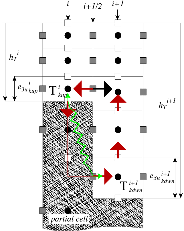
FIG. 5.4: Advective/diffusive Bottom Boundary Layer. The BBL parameterisation is activated when \rho_{kup}^i is larger than \rho_{kdwn}^{i+1} . Red arrows indicate the additional overturning circulation due to the advective BBL. The transport of the downslope flow is defined either as the transport of the bottom ocean cell (black arrow), or as a function of the along slope density gradient. The green arrow indicates the diffusive BBL flux directly connecting kup and kdwn ocean bottom cells. connection
