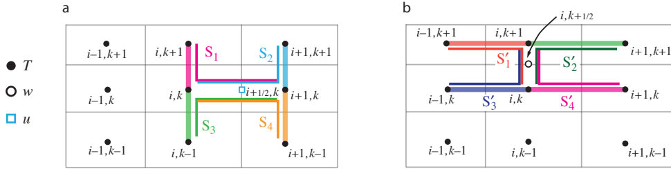
FIG. E.1: (a) Arrangement of triads S_i and tracer gradients to give lateral tracer flux from box i, k to i + 1, k (b) Triads S'_i and tracer gradients to give vertical tracer flux from box i, k to i, k + 1 .
