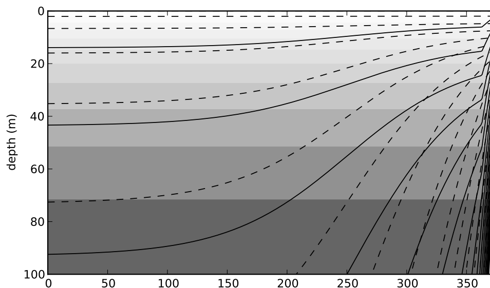
Figure 4.8: A comparison of the ? S -coordinate (solid lines), a 50 level Z -coordinate (contoured surfaces) and the ? S -coordinate (dashed lines) in the surface 100m for an idealised bathymetry that goes from 50m to 5500m depth. For clarity every third coordinate surface is shown.
