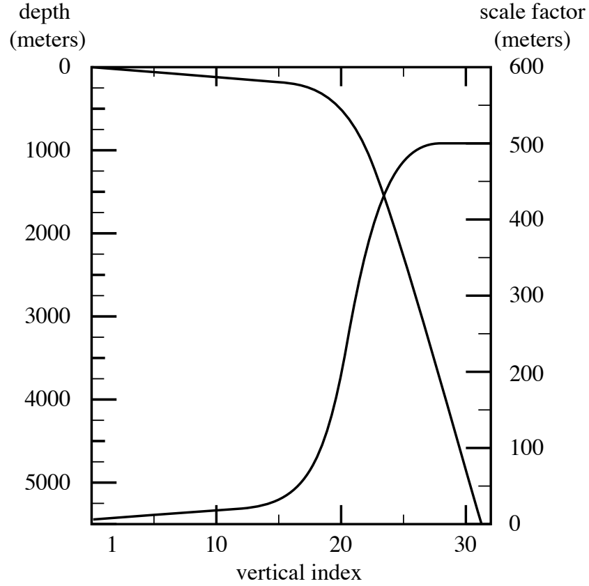
Figure 4.6: Default vertical mesh for ORCA2: 30 ocean levels (L30). Vertical level functions for (a) T-point depth and (b) the associated scale factor as computed from (??) using (??) in z -coordinate.
