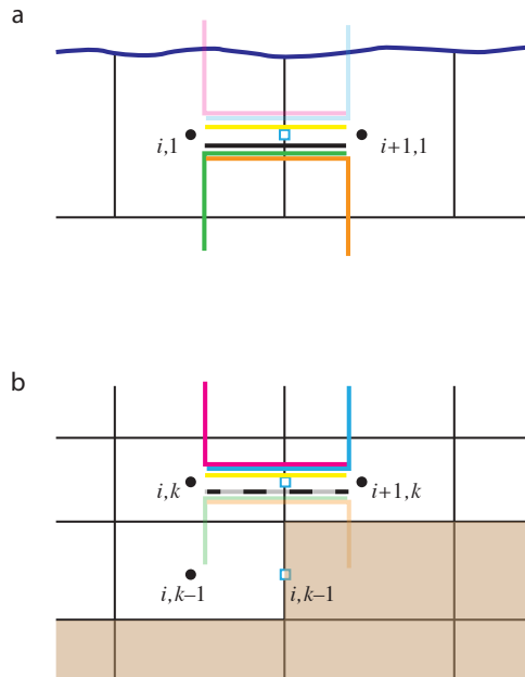
Figure D.3: (a) Uppermost model layer k = 1 with i, 1 and i + 1, 1 tracer points (black dots), and i + 1/2, 1 u -point (blue square). Triad slopes ^1_{i-1/2}\mathbb{R}_{1/2}^{-1/2} (magenta) and ^1_{i+1/2}\mathbb{R}_{-1/2}^{-1/2} (blue) poking through the ocean surface are masked (faded in figure). However, the lateral _{11} contributions towards ^1_{i-1/2}\mathbb{F}_{u_{1/2}}^{-1/2} and ^1_{i+1/2}\mathbb{F}_{u_{-1/2}}^{-1/2} (yellow line) are still applied, giving diapycnal diffusive fluxes. (b) Both near bottom triad slopes ^k_{i-1/2}\mathbb{R}_{1/2}^{1/2} and ^k_{i+1/2}\mathbb{R}_{-1/2}^{1/2} are masked when either of the i, k+1 or i+1, k+1 tracer points is masked, i.e. the i, k+1 u -point is masked. The associated lateral fluxes (grey-black dashed line) are masked if botmix_triad=false , but left unmasked, giving bottom mixing, if botmix_triad=true .
