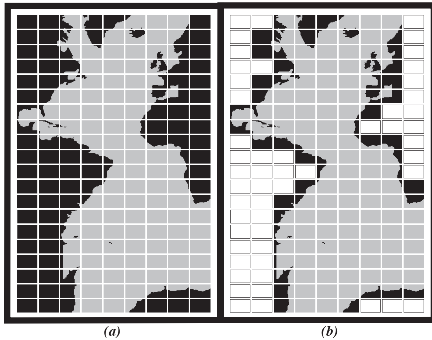
Figure 8.6: Example of Atlantic domain defined for the CLIPPER projet. Initial grid is composed of 773 x 1236 horizontal points. (a) the domain is split onto 9 subdomains ( jpm=9 , jpnj=20 ). 52 subdomains are land areas. (b) 52 subdomains are eliminated (white rectangles) and the resulting number of processors really used during the computation is jpmj=128 .
