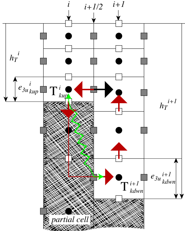
Figure 5.4: Advective/diffusive Bottom Boundary Layer. The BBL parameterisation is activated when \rho_{kup}^i is larger than \rho_{kdwn}^{i+1} . Red arrows indicate the additional overturning circulation due to the advective BBL. The transport of the downslope flow is defined either as the transport of the bottom ocean cell (black arrow), or as a function of the along slope density gradient. The green arrow indicates the diffusive BBL flux directly connecting kup and kdwn ocean bottom cells. connection
