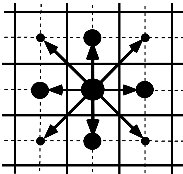
Figure 9.1: averaging procedure for isopycnal slope computation.
