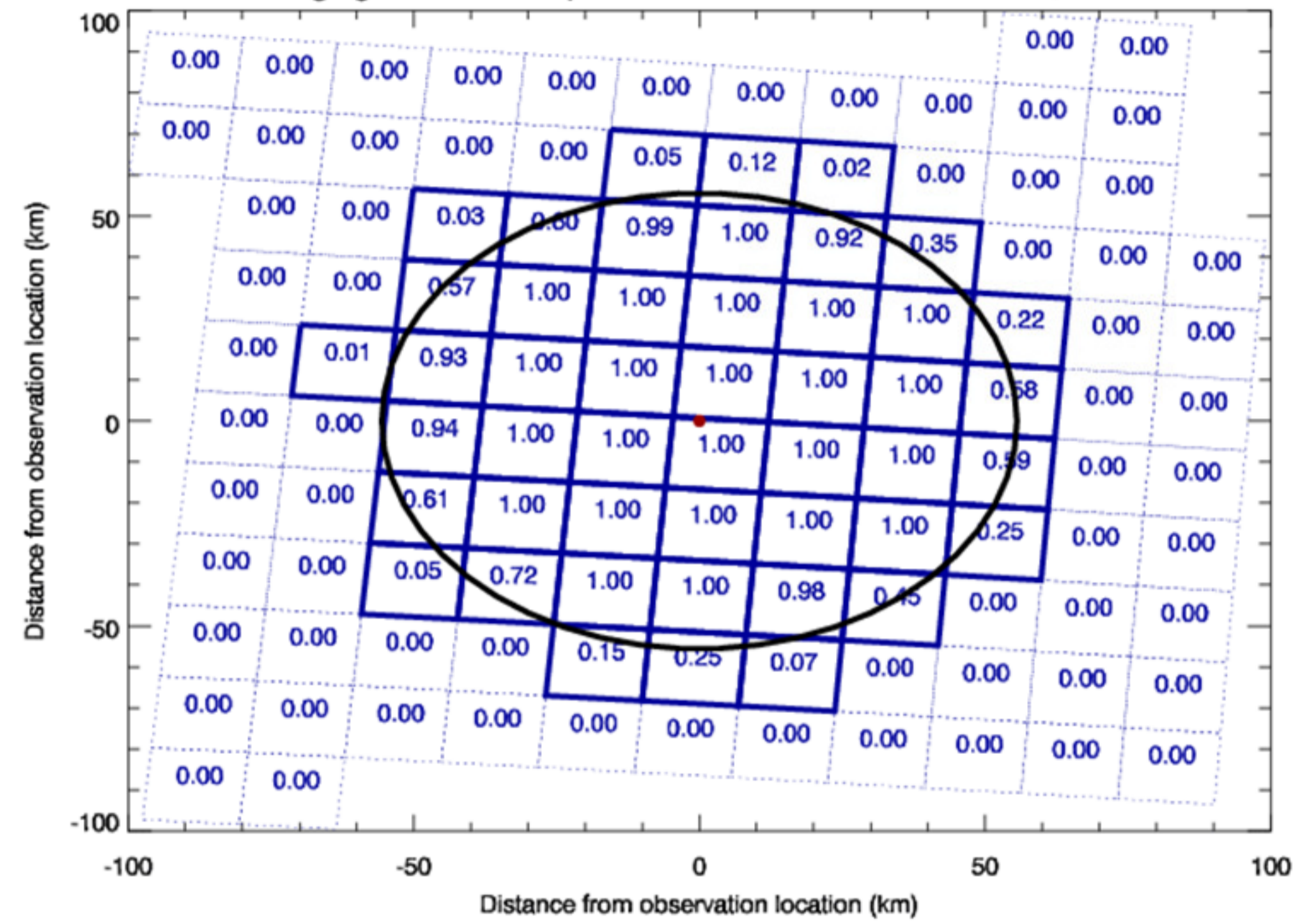
Averaging observation operator for ob centred on: -173.50E, 56.00N
