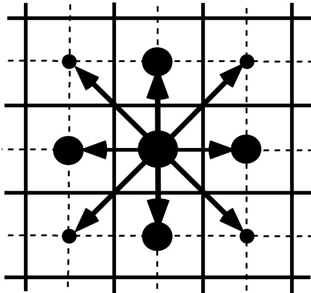
FIG. 9.1: averaging procedure for isopycnal slope computation.
