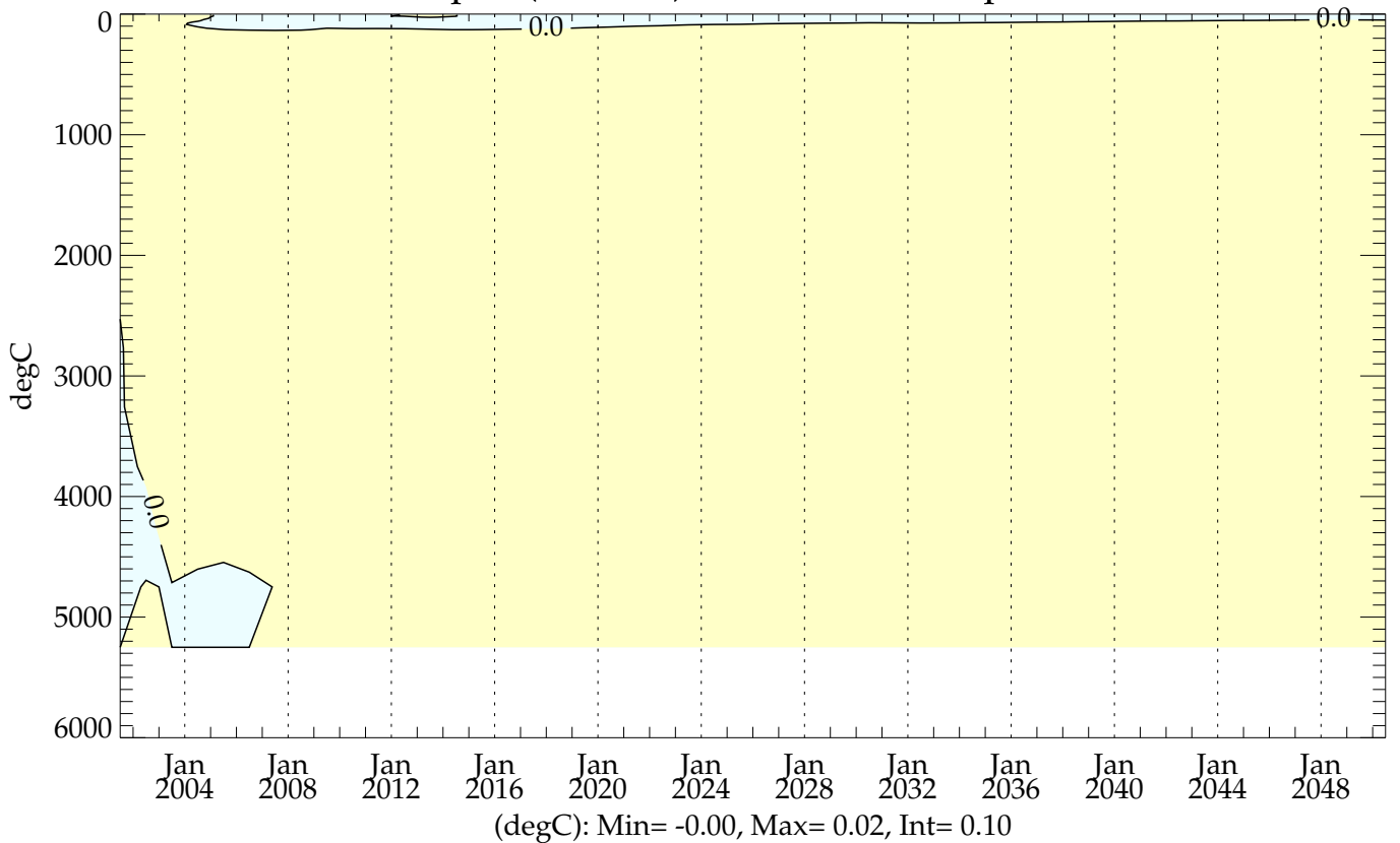
hic005 - testht (20010101 - 20501231) ZT-plot (0-6000m) Global Mean Temperature
