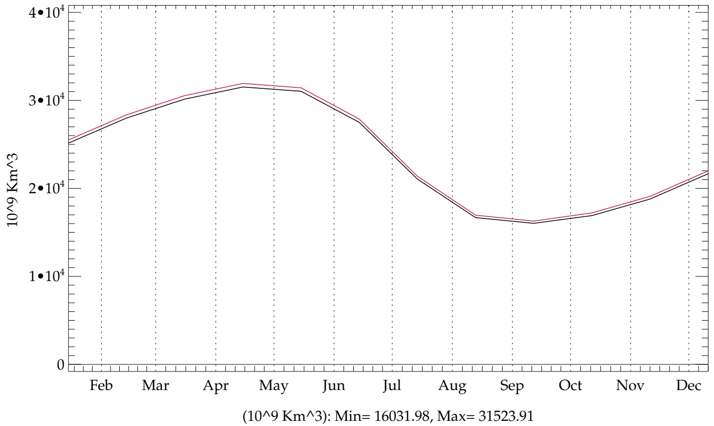
Northern Hemisphere hic005 (BLACK) - testht (RED) (20010101 - 20501231) Global Annual Mean Ice Volume (BLACK)
