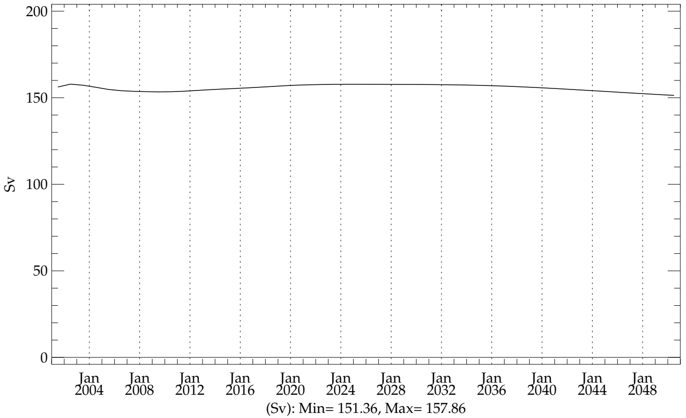
hic005 (20010101 - 20501231) Drake Transport
