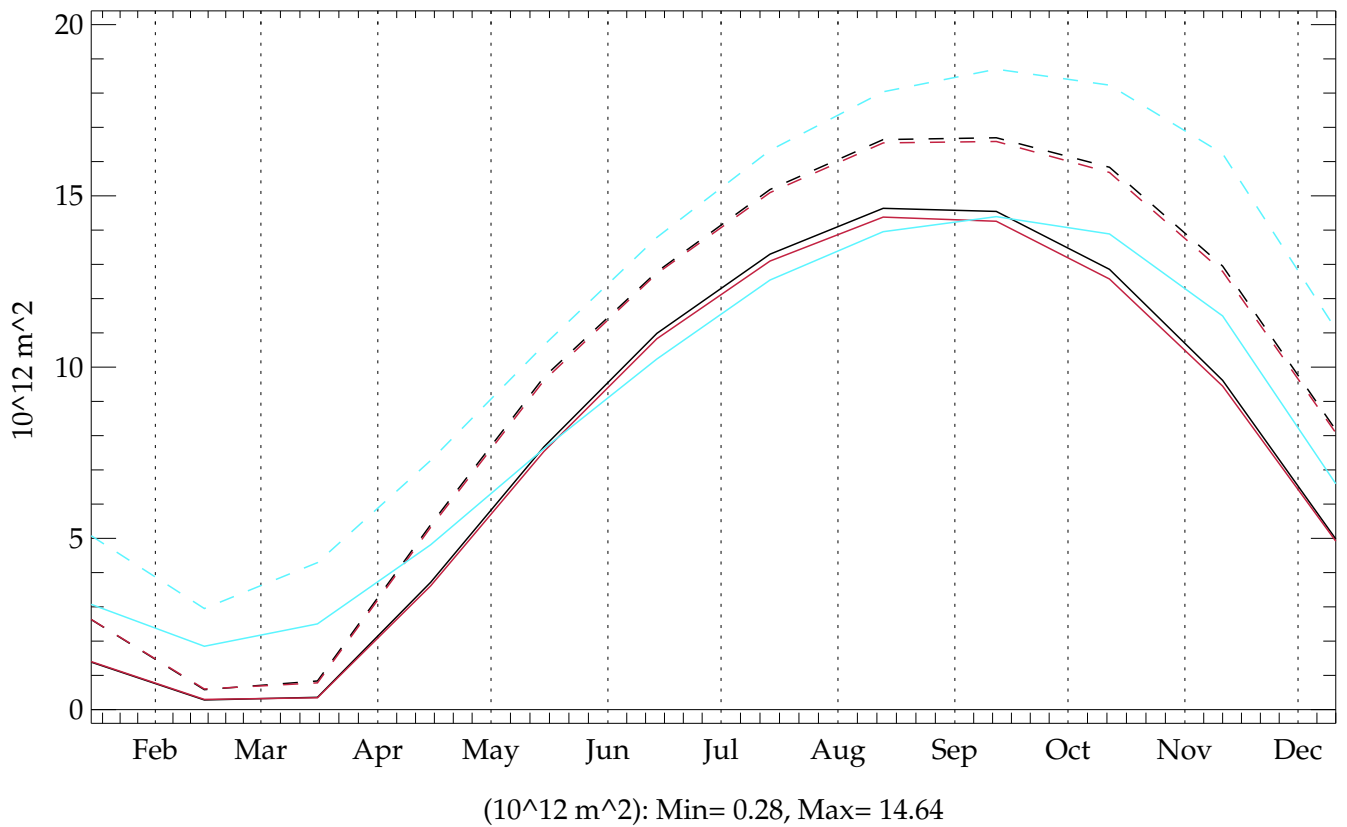
Southern Hemisphere hic005 (BLACK) - testht (RED) (20010101 - 20501231) OBSERVATION (light blue) Global Annual Mean Ice Area (CONTINUOUS) and Extend minus 15% (DASHED)
