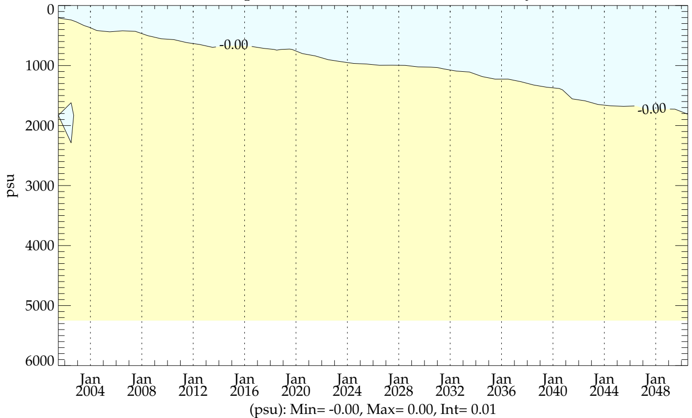
hic005 - testht (20010101 - 20501231) ZT-plot (0-6000m) Global Mean Salinity
