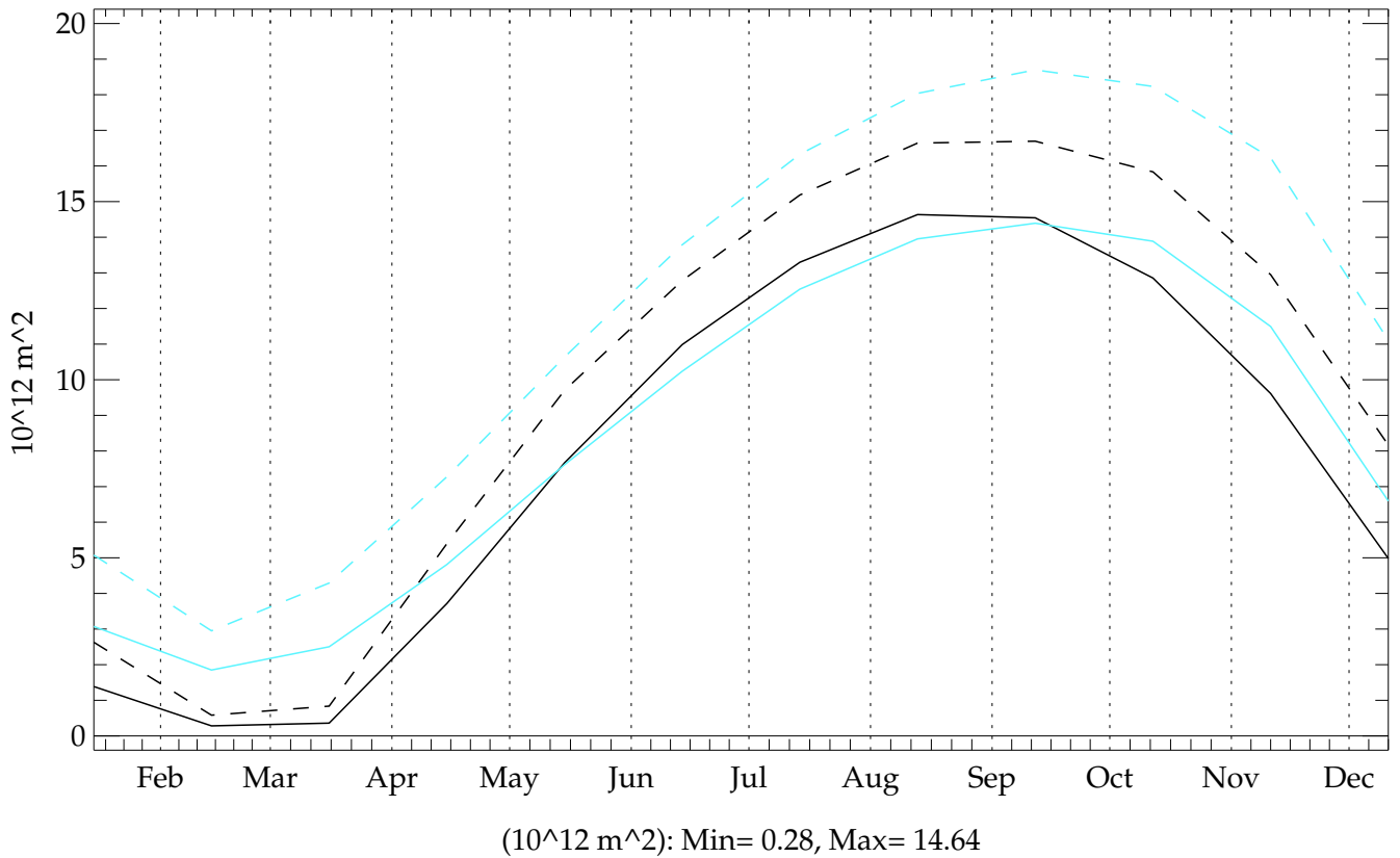
Southern Hemisphere hic005 (BLACK) (20010101 - 20501231) OBSERVATION (light blue) Global Annual Mean Ice Area (CONTINUOUS) and Extend minus 15% (DASHED)
