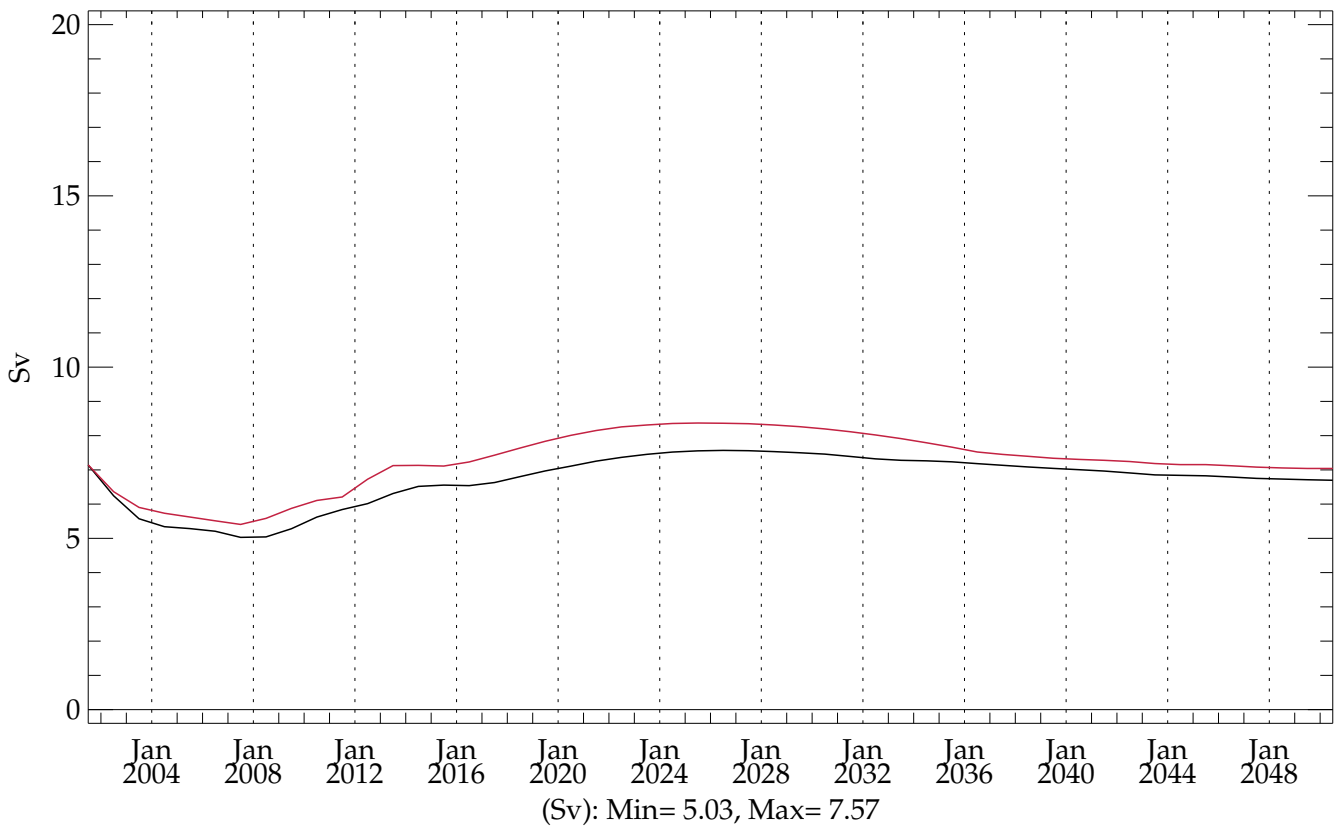
hic005 (BLACK) - testht (RED) (20010101 - 20501231) Max AntArctic Bottom Water between 80S and 65S
