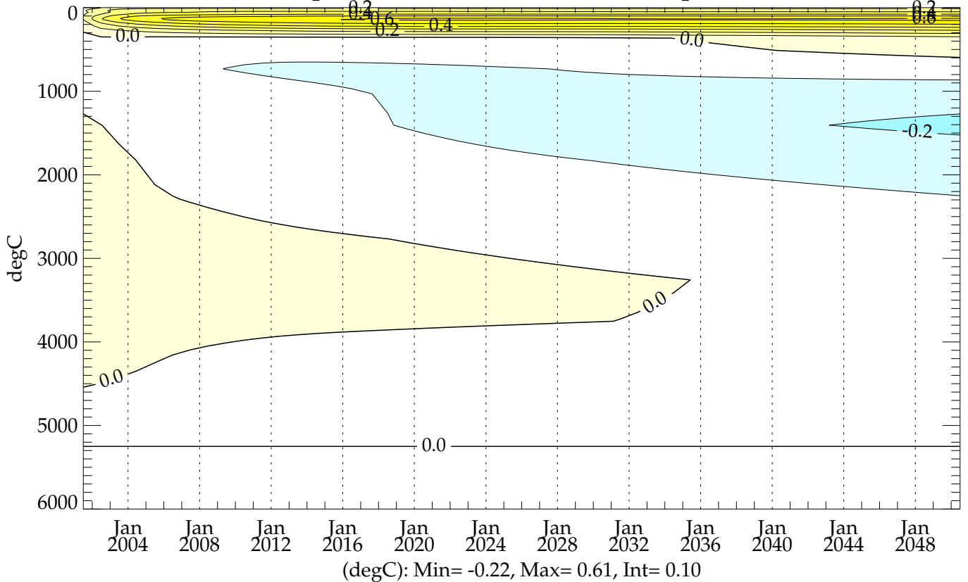
hic005 (20010101 - 20501231) - Levitus ZT-plot (0-6000m) Global Mean Temperature
