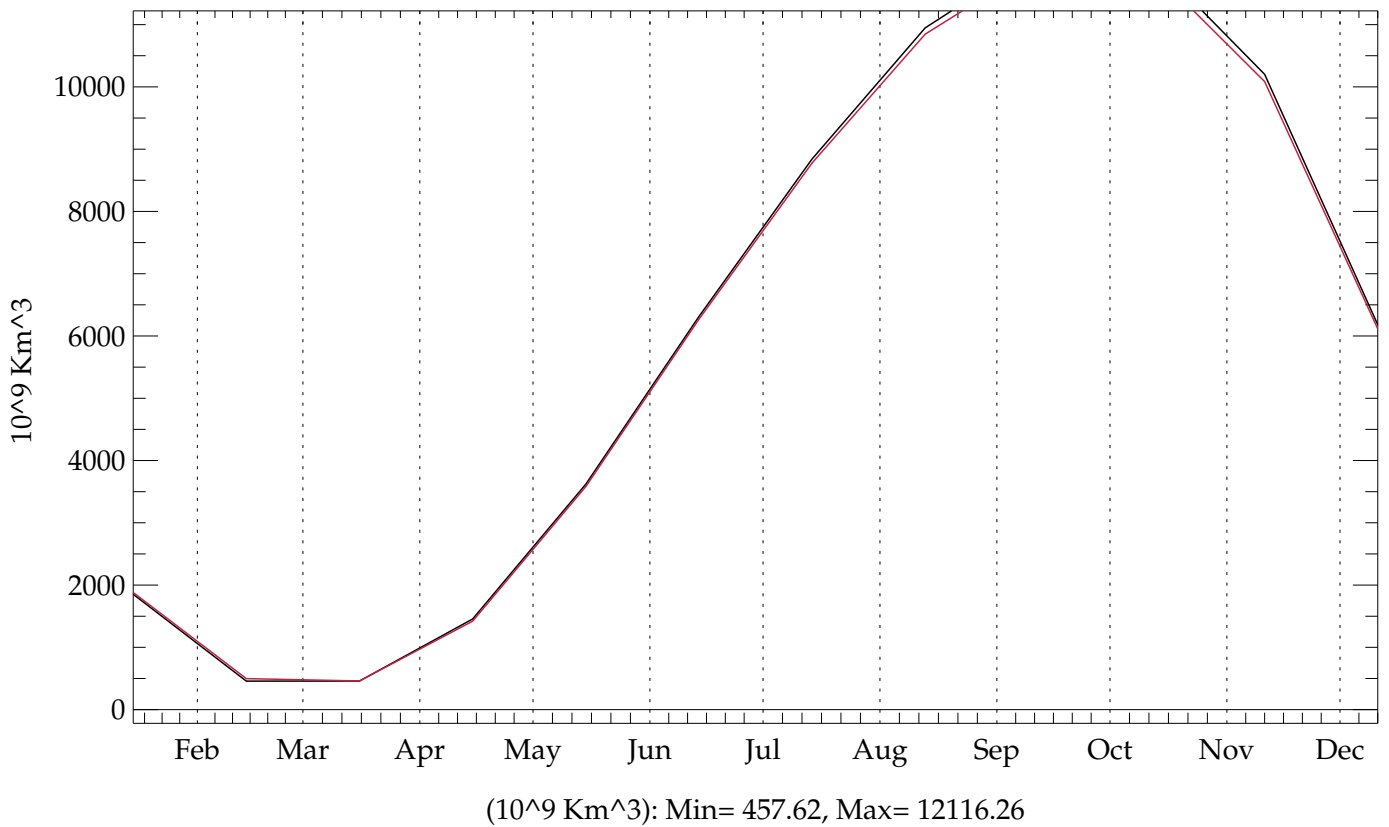
Southern Hemisphere hic005 (BLACK) - testht (RED) (20010101 - 20501231) Global Annual Mean Ice Volume
