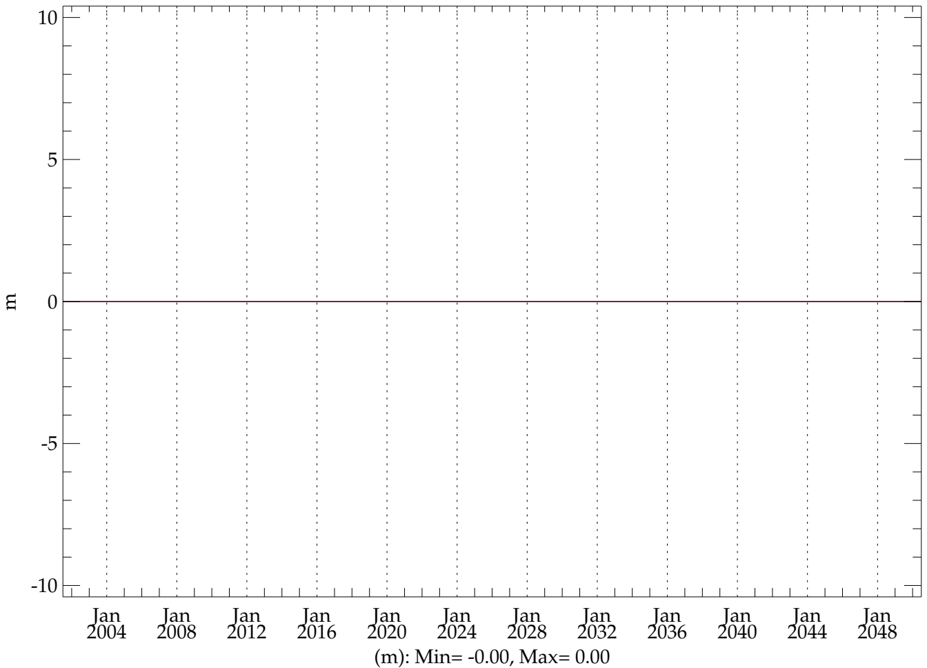
hic005 (BLACK) - testht (RED) (20010101 - 20501231) Global Mean SSH
