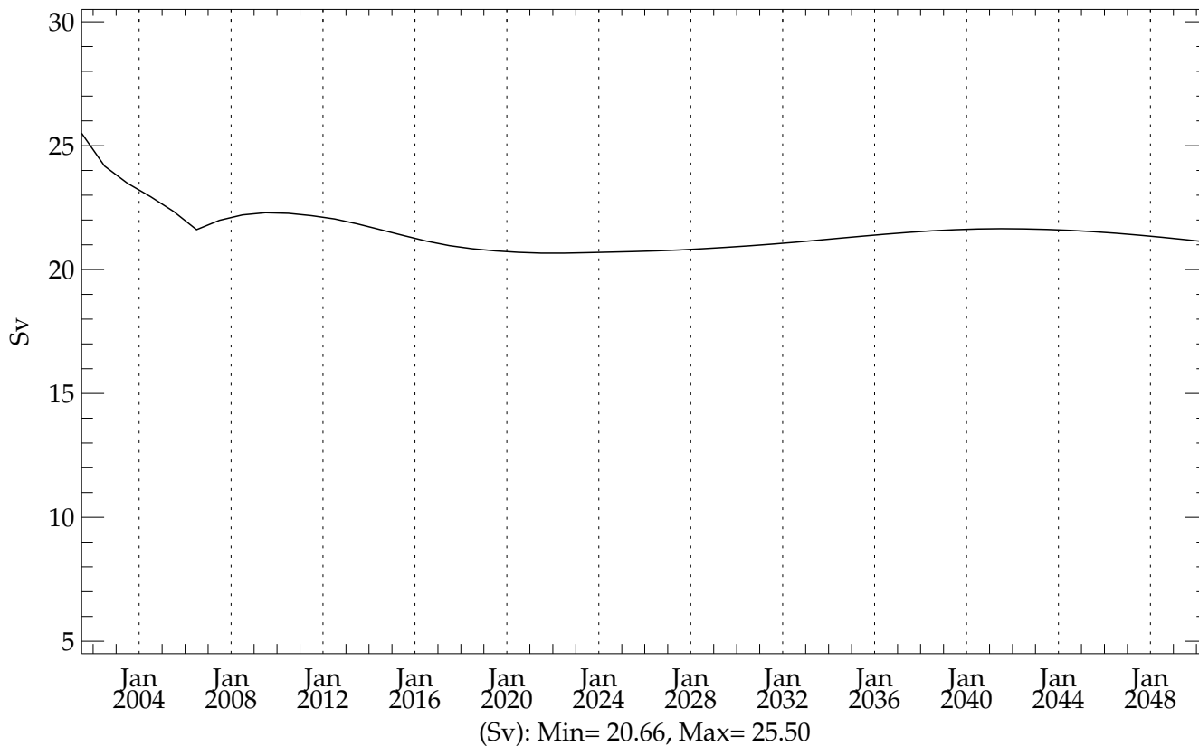
hic005 (20010101 - 20501231) Max AntArctic Bottom Cell between 65S and 30N (20010101 - 20501231)
