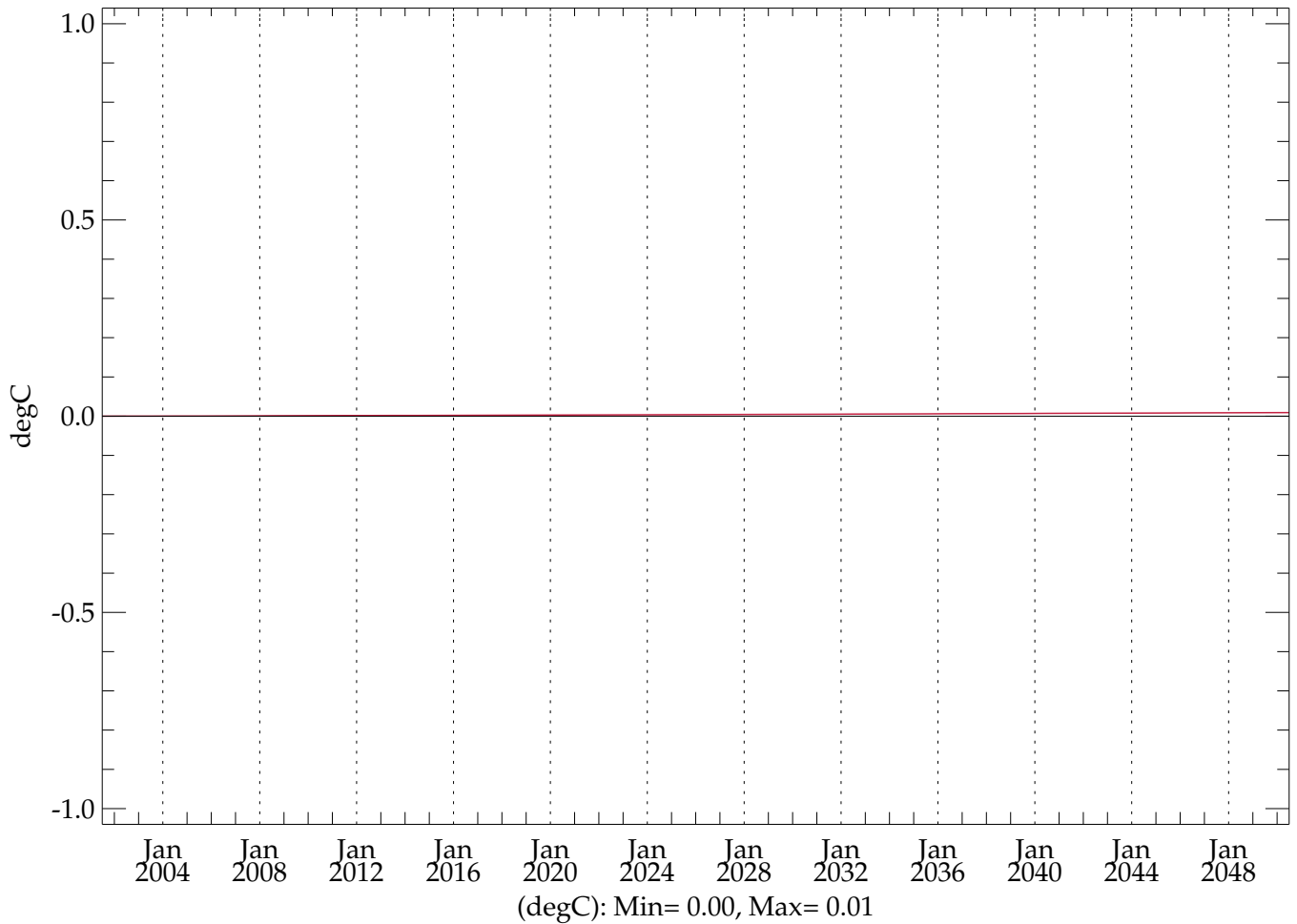
hic005 - testht (20010101 - 20501231) ZT-plot (0-6000m) Global Mean Temperature
