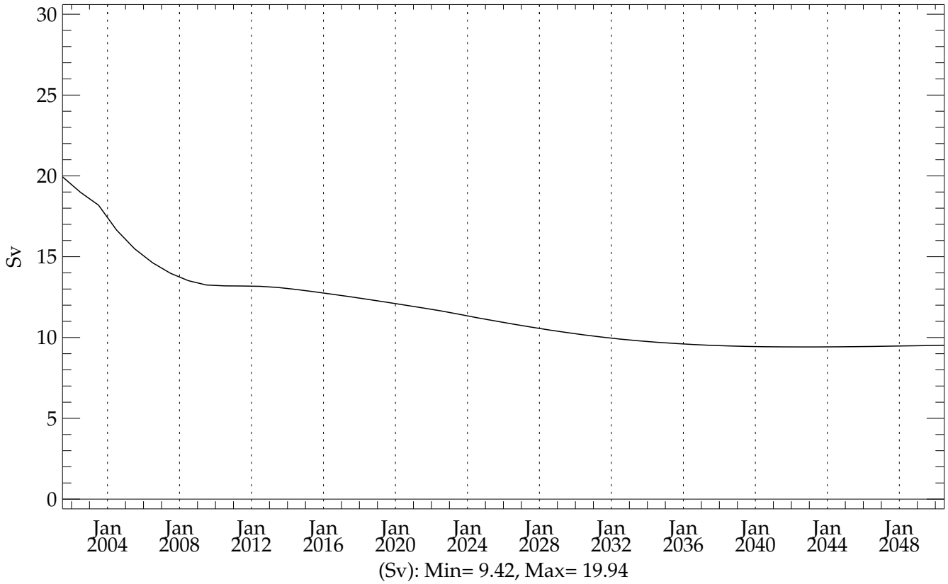
hic005 (20010101 - 20501231) Max Atlantic MOC between 40N and 50N
