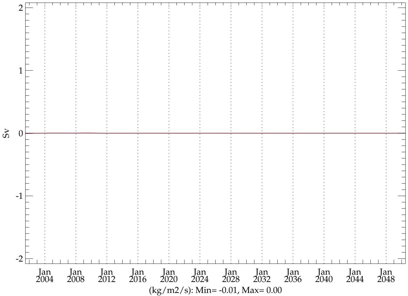
hic005 (BLACK) - testht (RED) (20010101 - 20501231) Global Mean EMP
