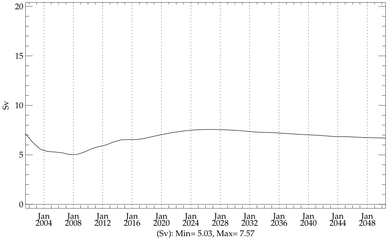
hic005 (20010101 - 20501231) Max AntArctic Bottom Water between 80S and 65S (20010101 - 20501231)
