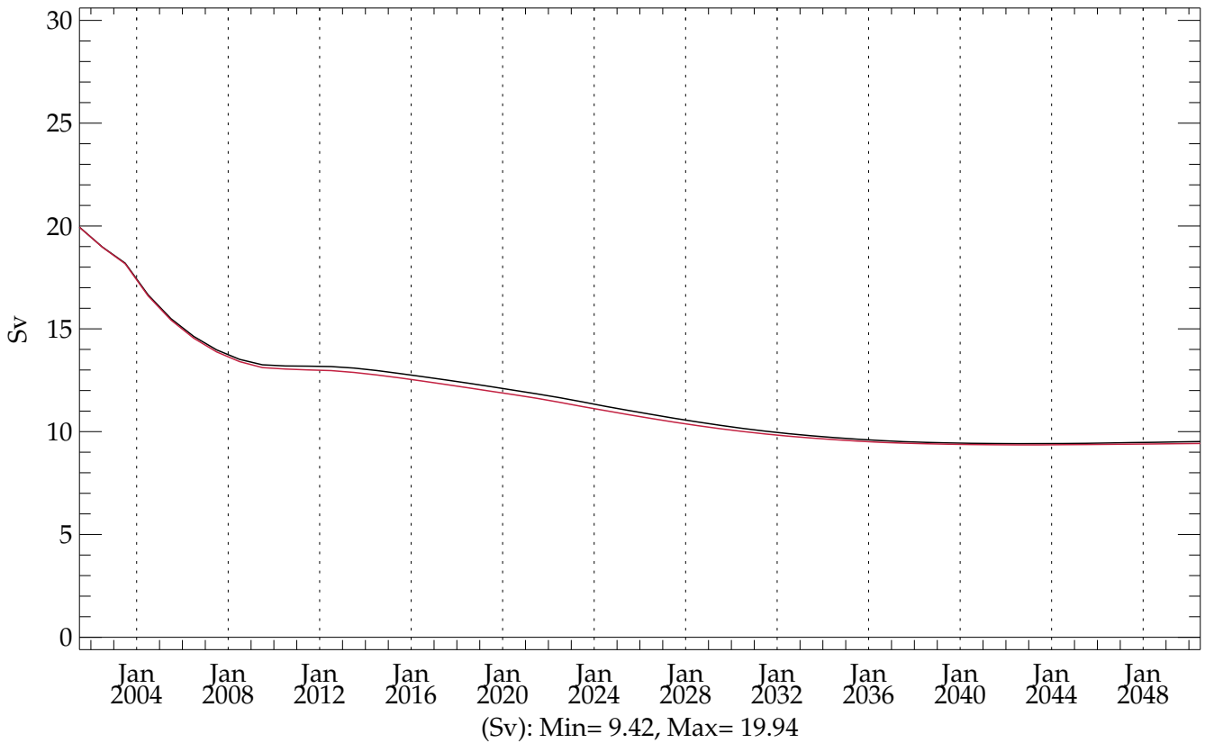
hic005 (BLACK) - testht (RED) (20010101 - 20501231) Max Atlantic MOC between 40N and 50N
