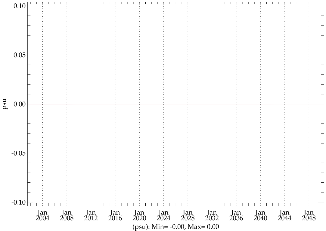
hic005 - testht (20010101 - 20501231) ZT-plot (0-6000m) Global Mean Salinity
