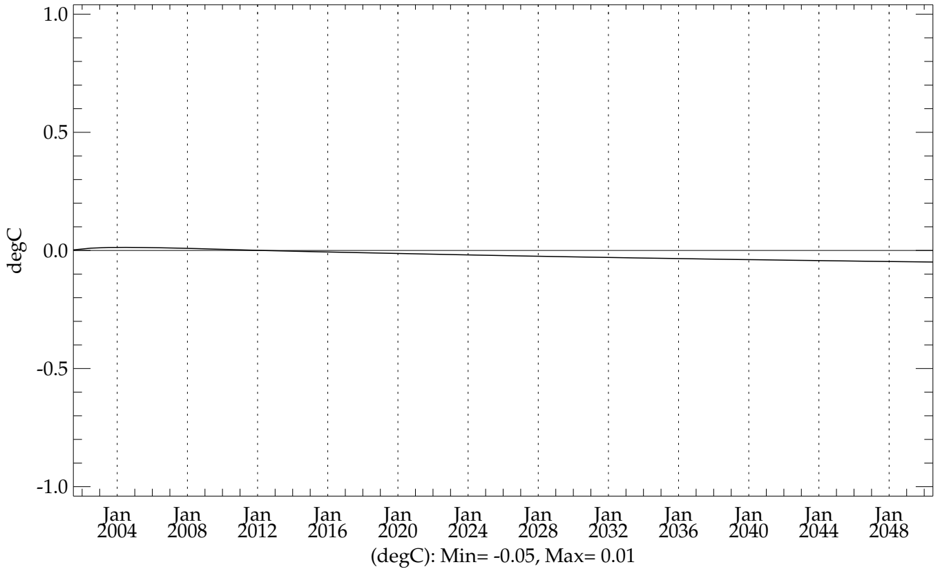
hic005 (20010101 - 20501231) - Levitus Global Mean Temperature
