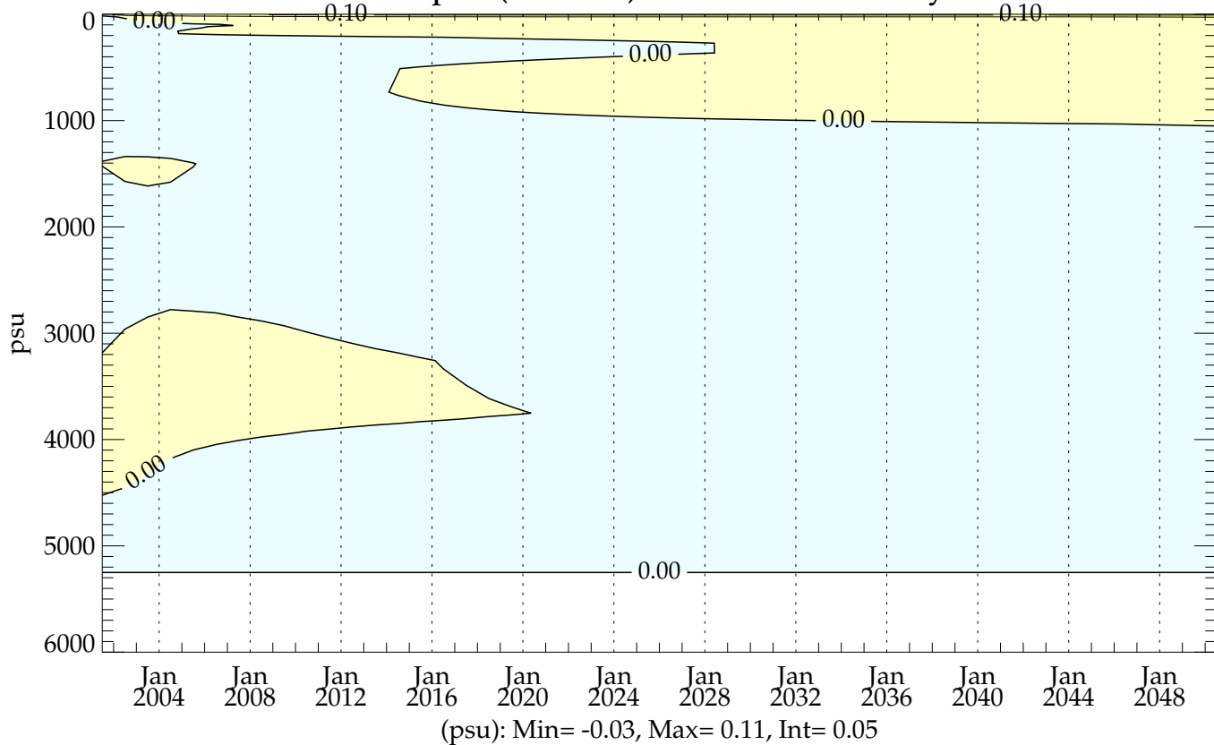
hic005 (20010101 - 20501231) - Levitus ZT-plot (0-6000m) Global Mean Salinity
