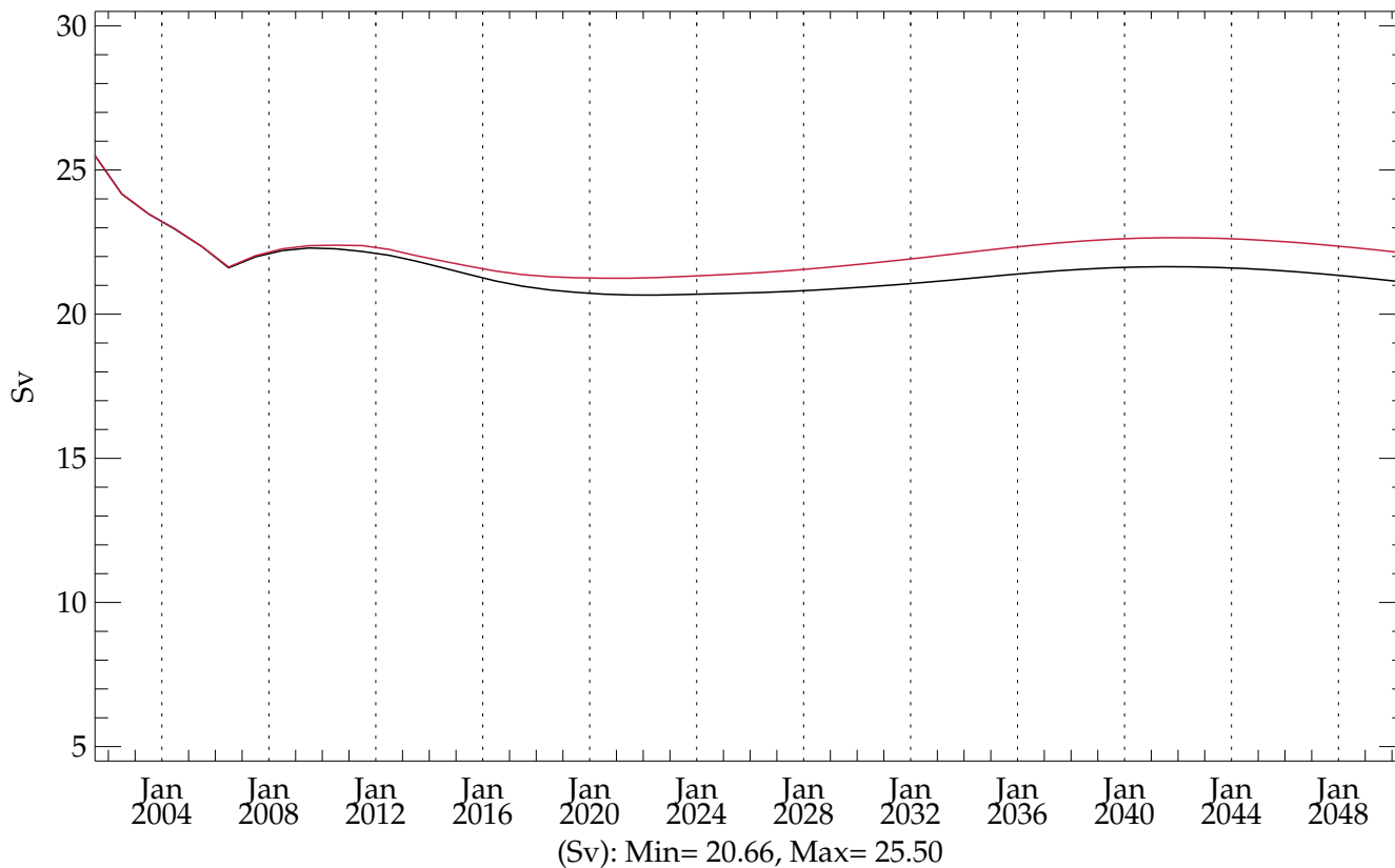
hic005 (BLACK) - testht (RED) (20010101 - 20501231) Max AntArctic Bottom Cell between 65S and 30N
