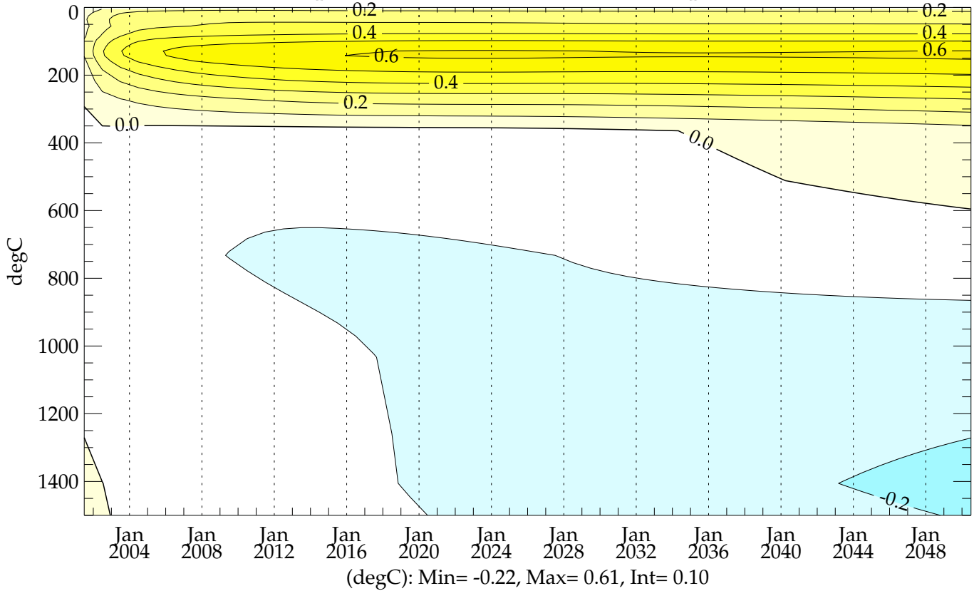
hic005 (20010101 - 20501231) - Levitus ZT-plot (0-1500m) Global Mean Temperature
