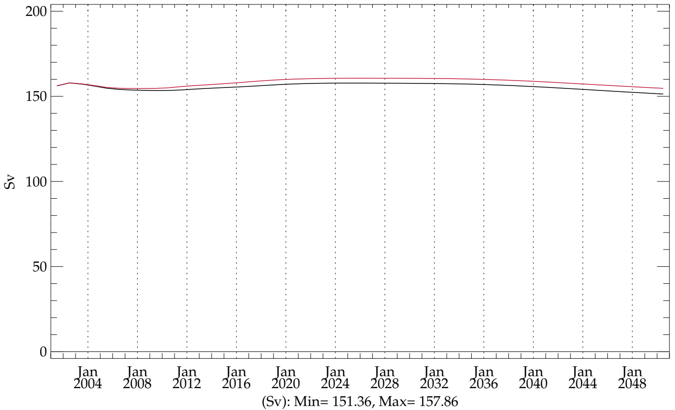
hic005 (BLACK) - testht (RED) (20010101 - 20501231) Drake Transport
