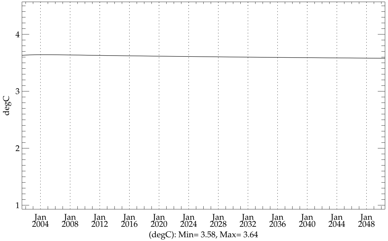
hic005 (20010101 - 20501231) Global Mean Temperature
