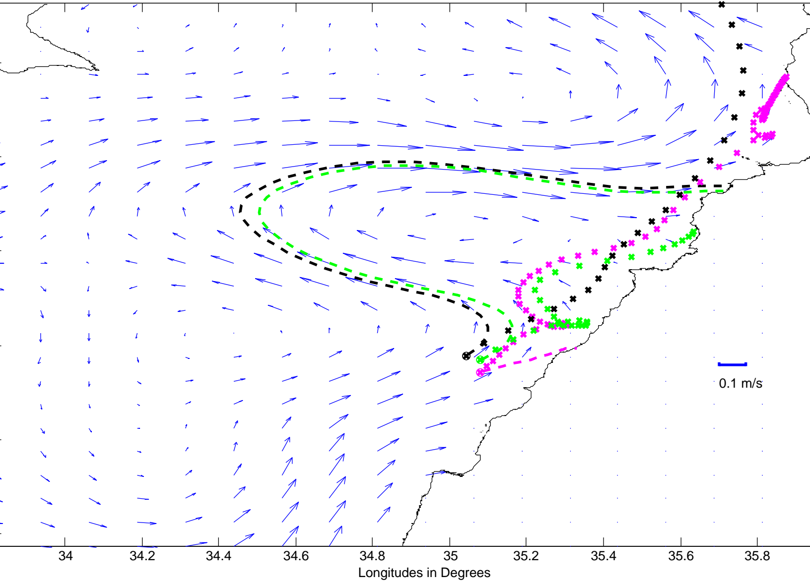
Altfloat Drifters vs Simulated (with AVISO) Trajectories starting on 28-08-13
