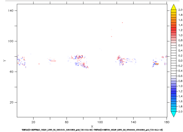
Standard isopycnal operator
